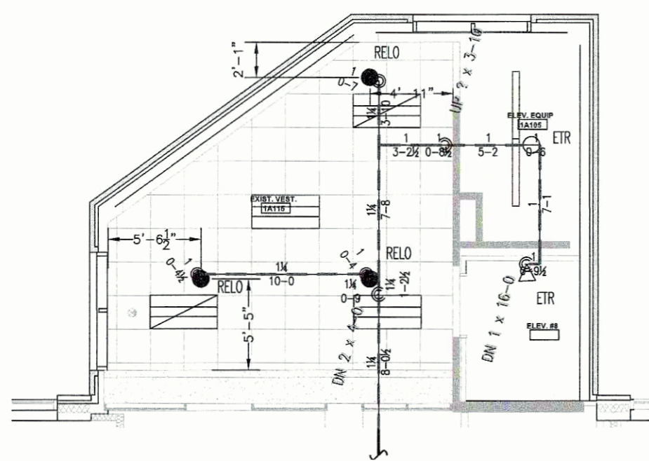
1ST FLOOR VESTIBULE SCALE: 1/8" = 1'-0"
