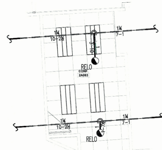
2nd FLOOR FIRE PROTECTION LAYOUT SCALE: 1/8" = 1'-0"
