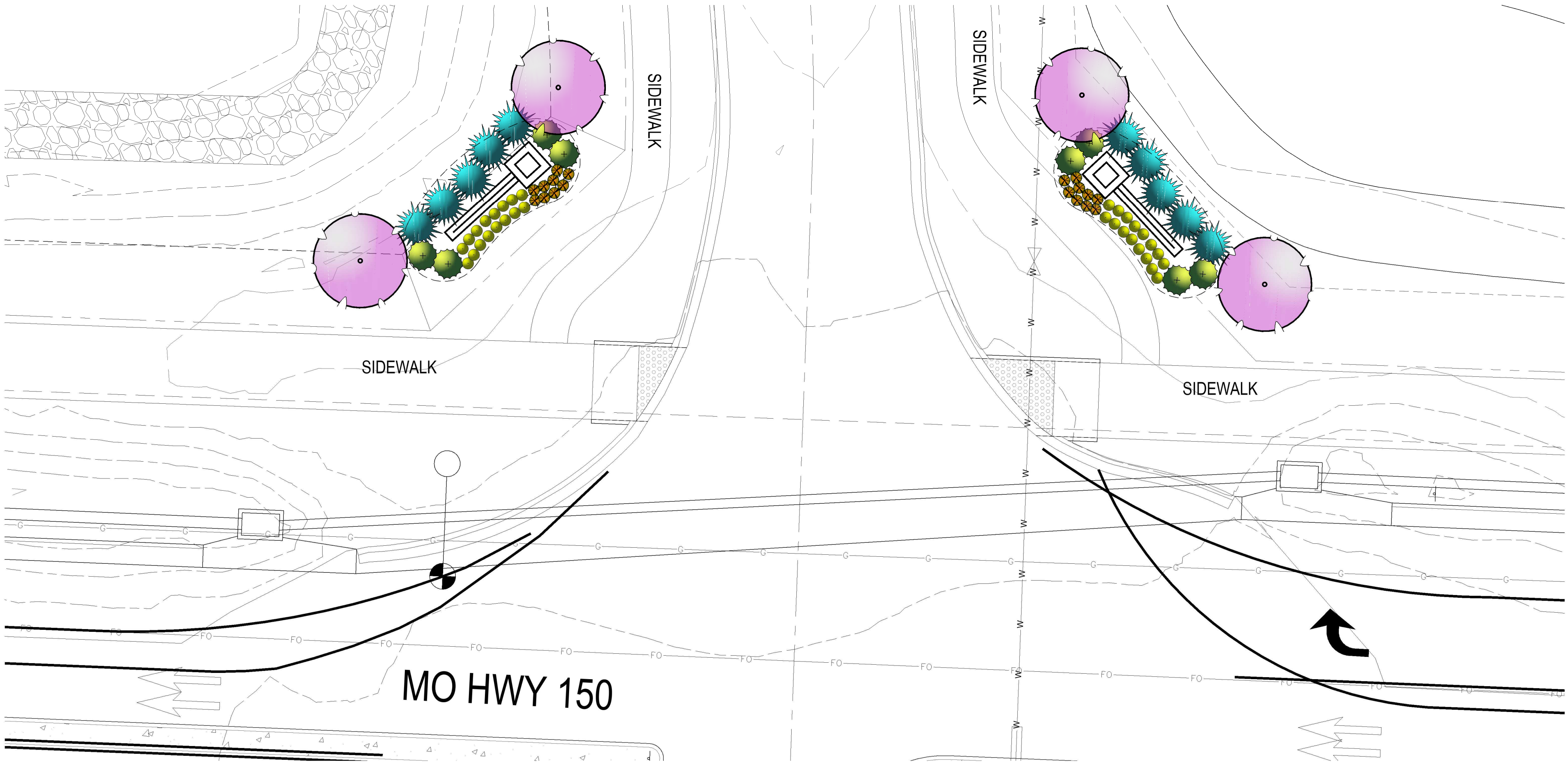
1 LANDSCAPE/LAYOUT PLAN (WEST MONUMENT) SCALE: 1"=10'-0"
