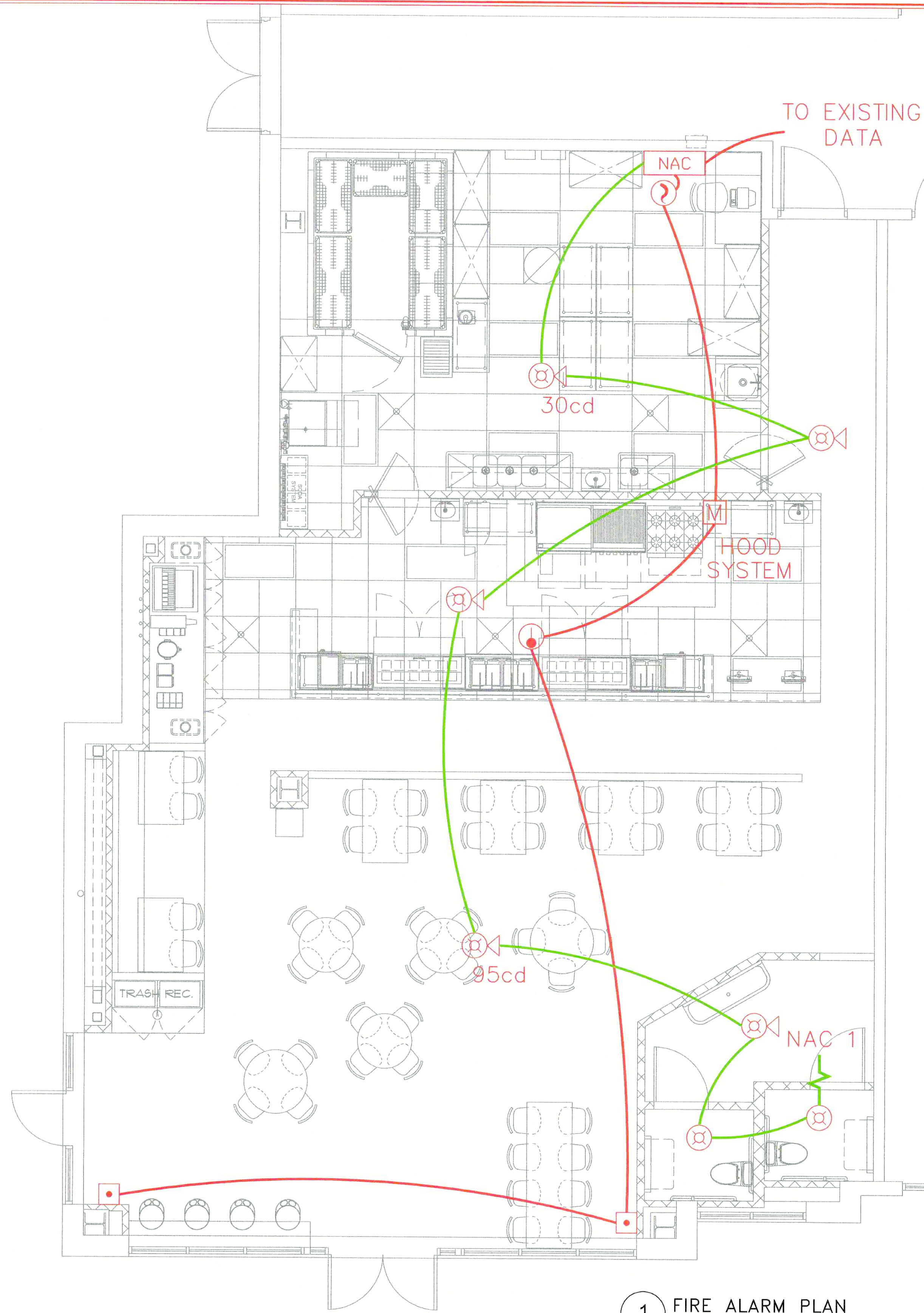
1 FIRE ALARM PLAN 1/4" = 1'0"
