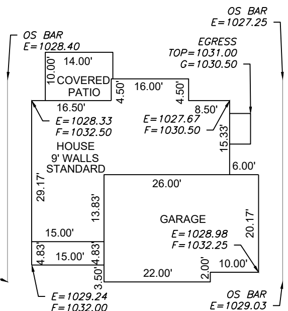
Scale 1"=20' PLAN: PRESTON RIDGE
