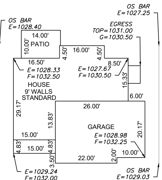
Scale 1"=20' PLAN: PRESTON RIDGE
