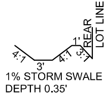
TYP. SWALE SECTION
