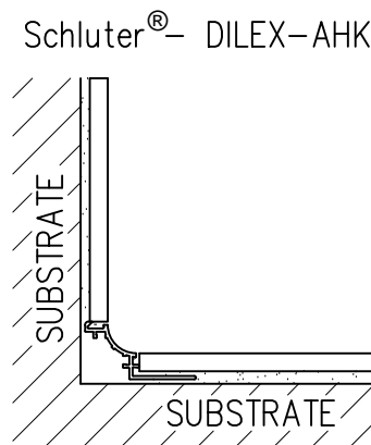
5 SCHLUTER BASE DETAIL NOT TO SCALE
