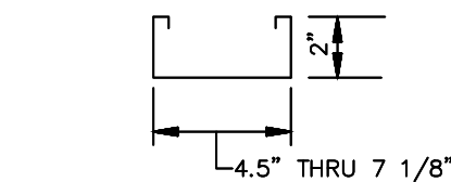
2" DOOR FRAME DETAIL
