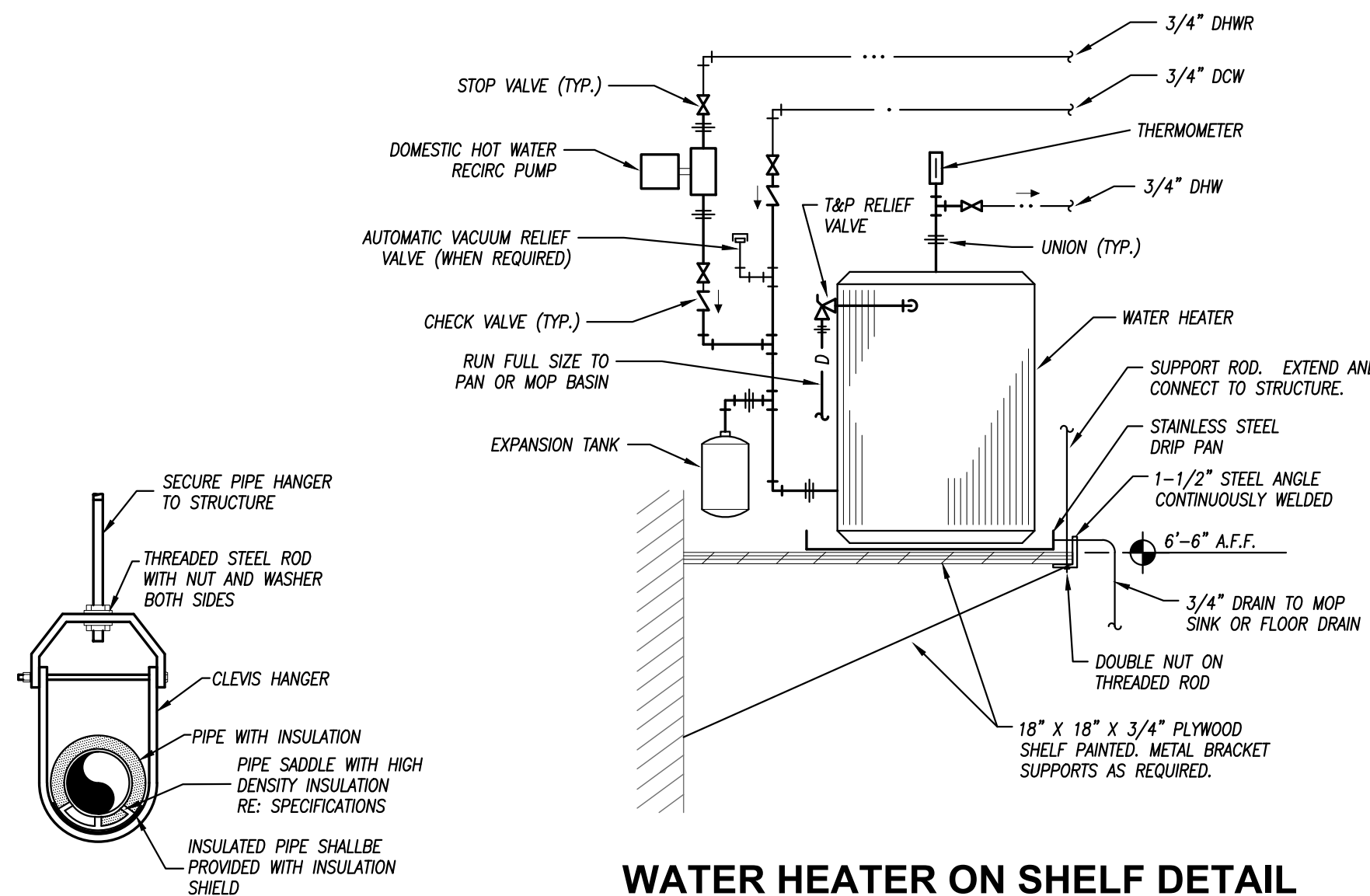
WATER HEATER ON SHELF DETAIL NOT TO SCALE
