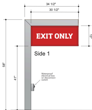
ELEVATION VIEW Scale: 3/4" = 1'-0" Area: 3.0 Sq.Ft.
