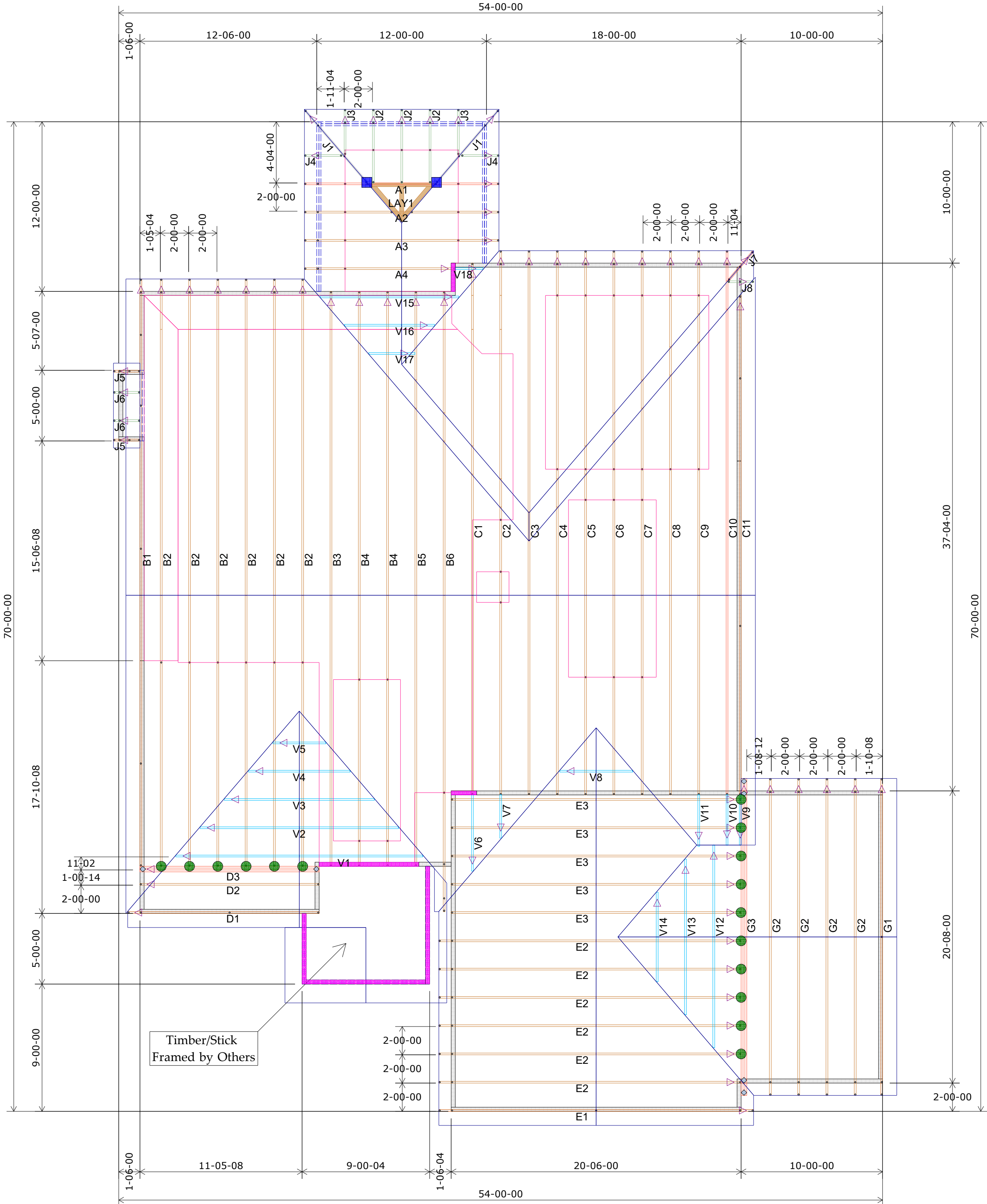
Roof Truss Layout Scale: 3/16" = 1'
