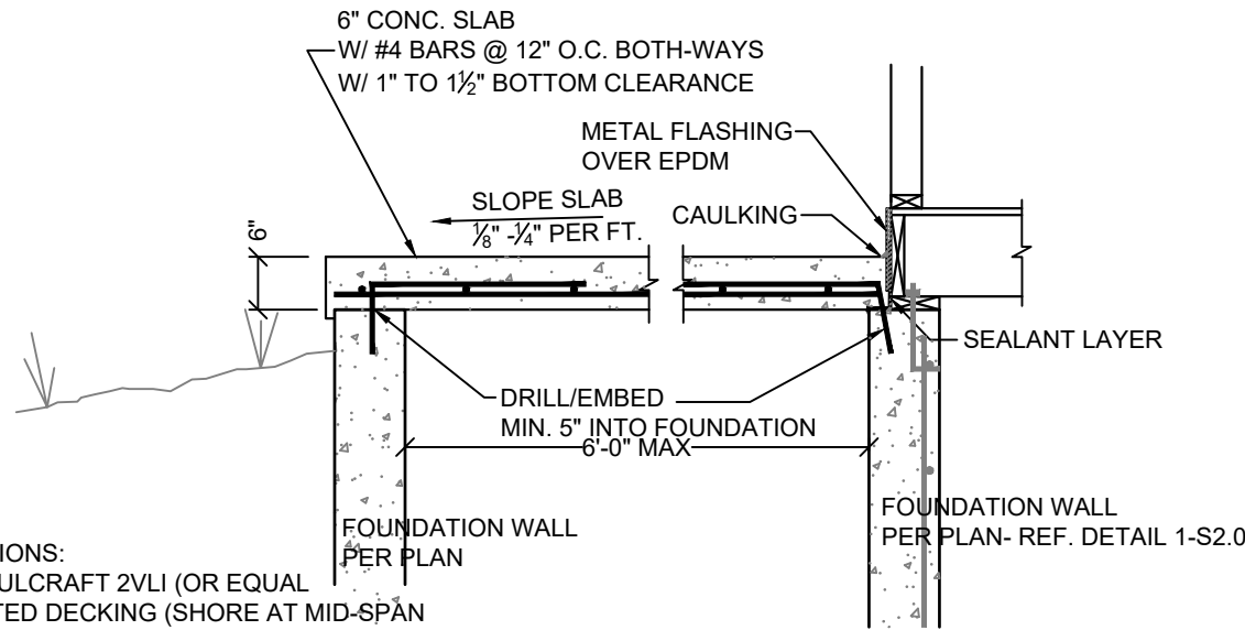
7 SUSPENDED PORCH STOOP DETAIL 1/2" = 1'-0"
