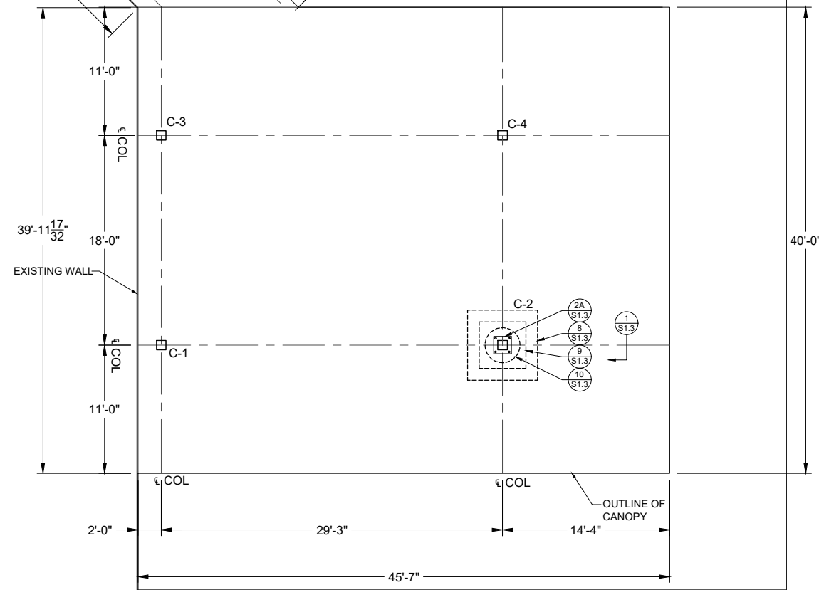
2 PROPOSED COLUMN LAYOUT SCALE: 1/4" = 1'-0"
