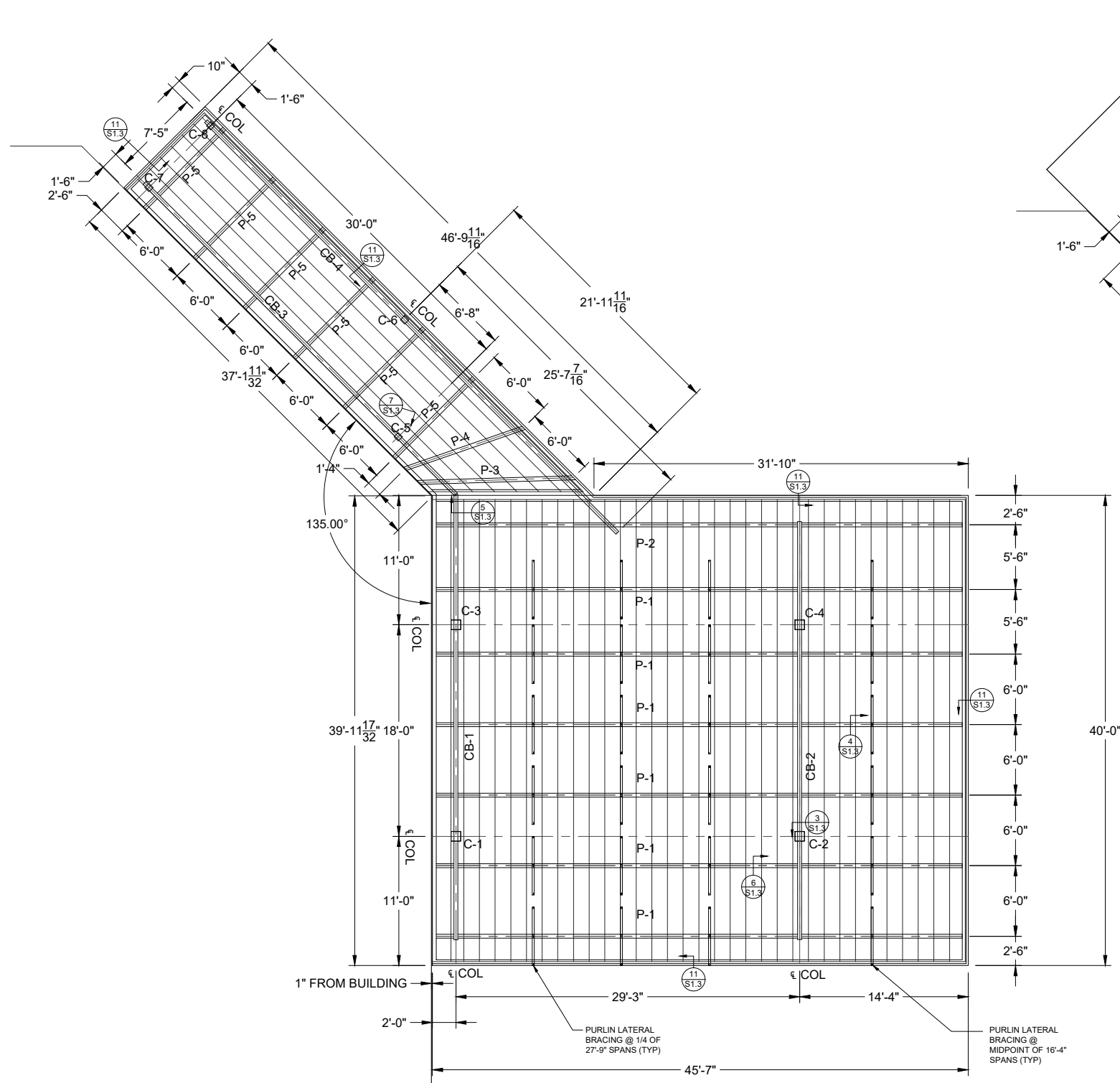
1 PROPOSED CANOPY LAYOUT SCALE: 1/4" = 1'-0"
