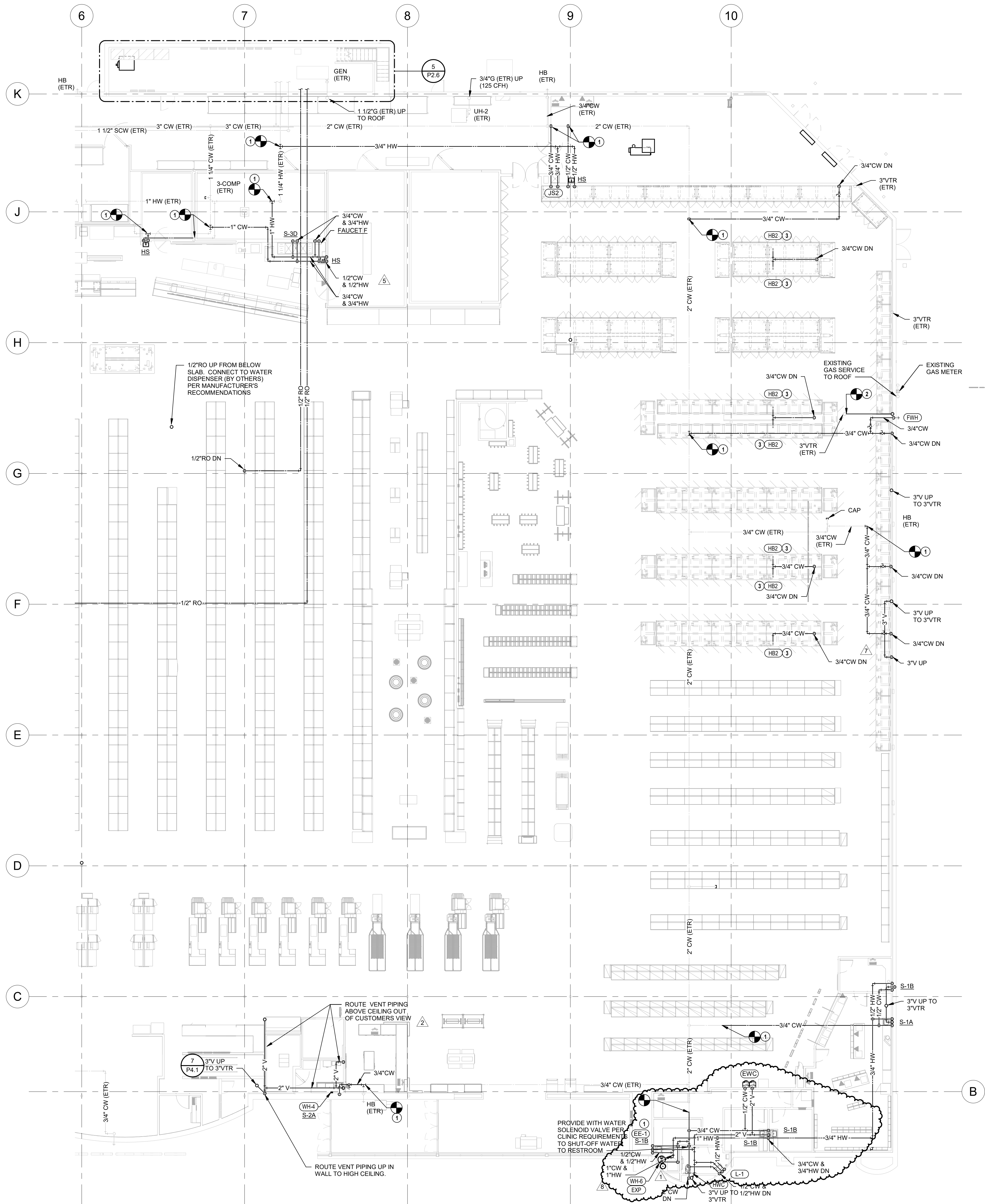
1 PLUMBING FLOOR PLAN - B 3/32" = 1'-0"
