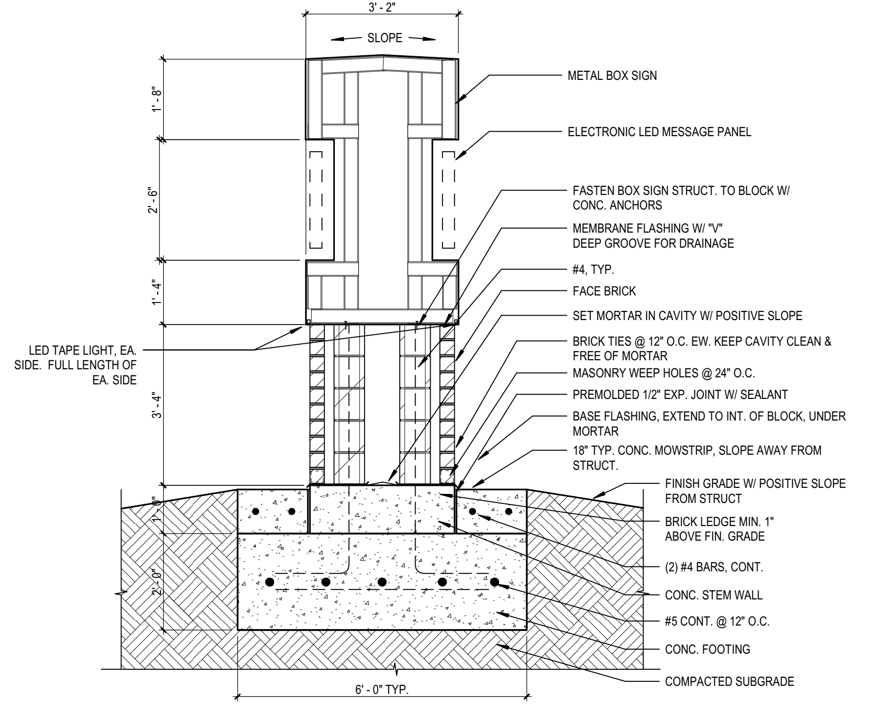
2 TYP. SIGN SECTION SCALE: 1/2" = 1'-0"
