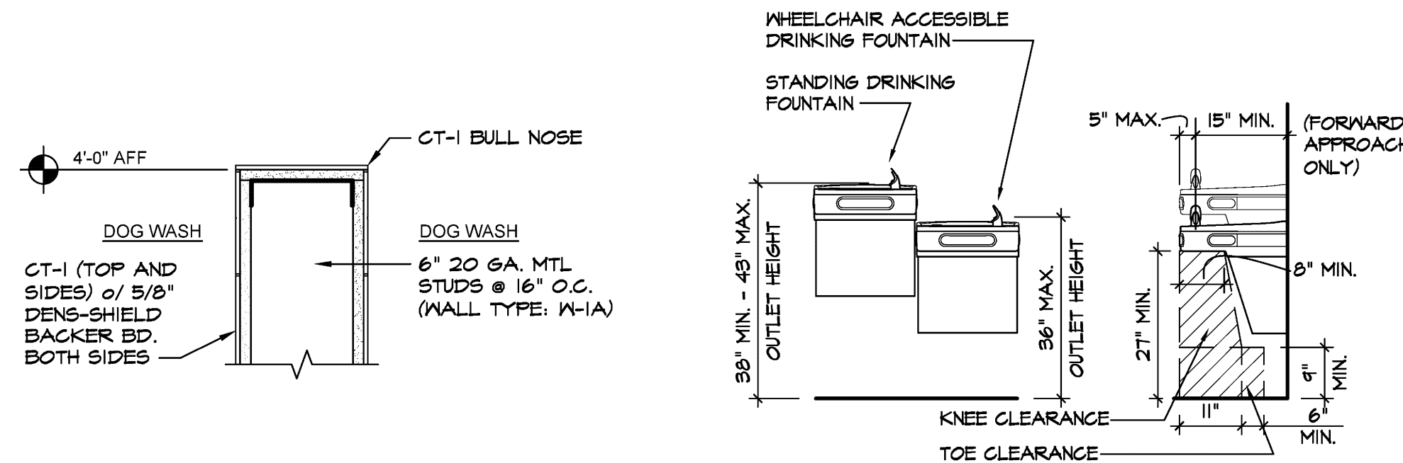
6 | ACCESSIBLE DRINKING FOUNTAIN ELEVATION 1/2"=1'-0"
