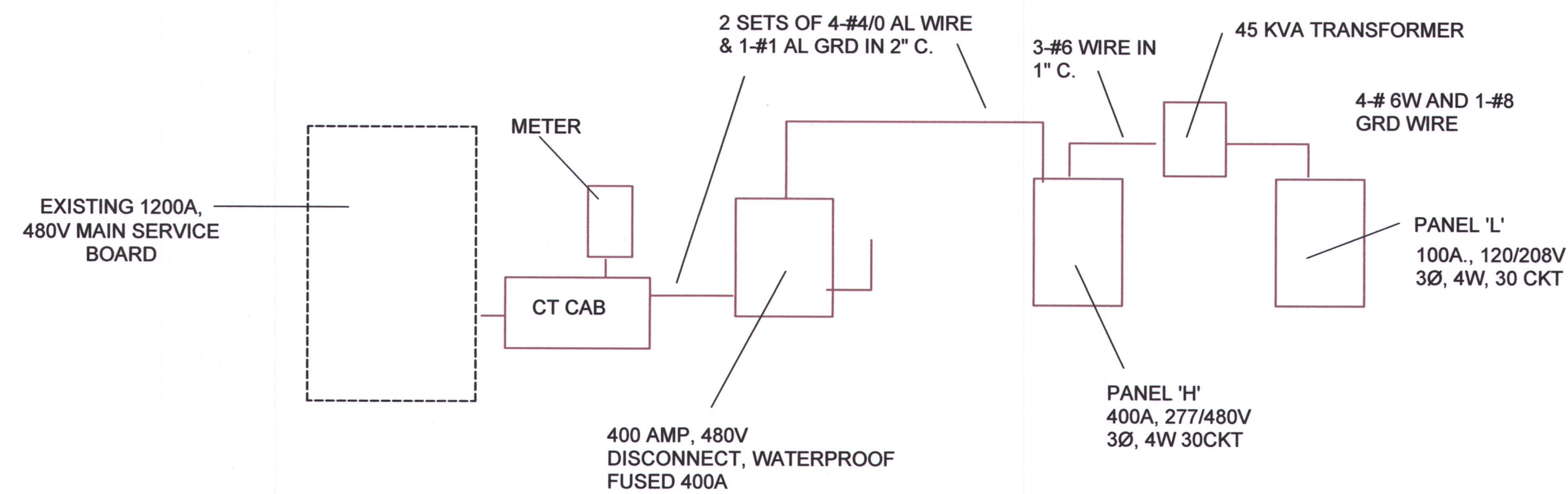
ELECTRICAL RISER DIAGRAM
