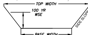
TYPICAL CHANNEL SECTION SWALE DETAIL
