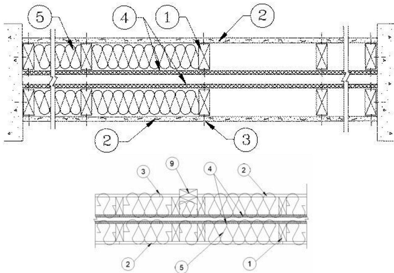
HORIZONTAL SECTION
