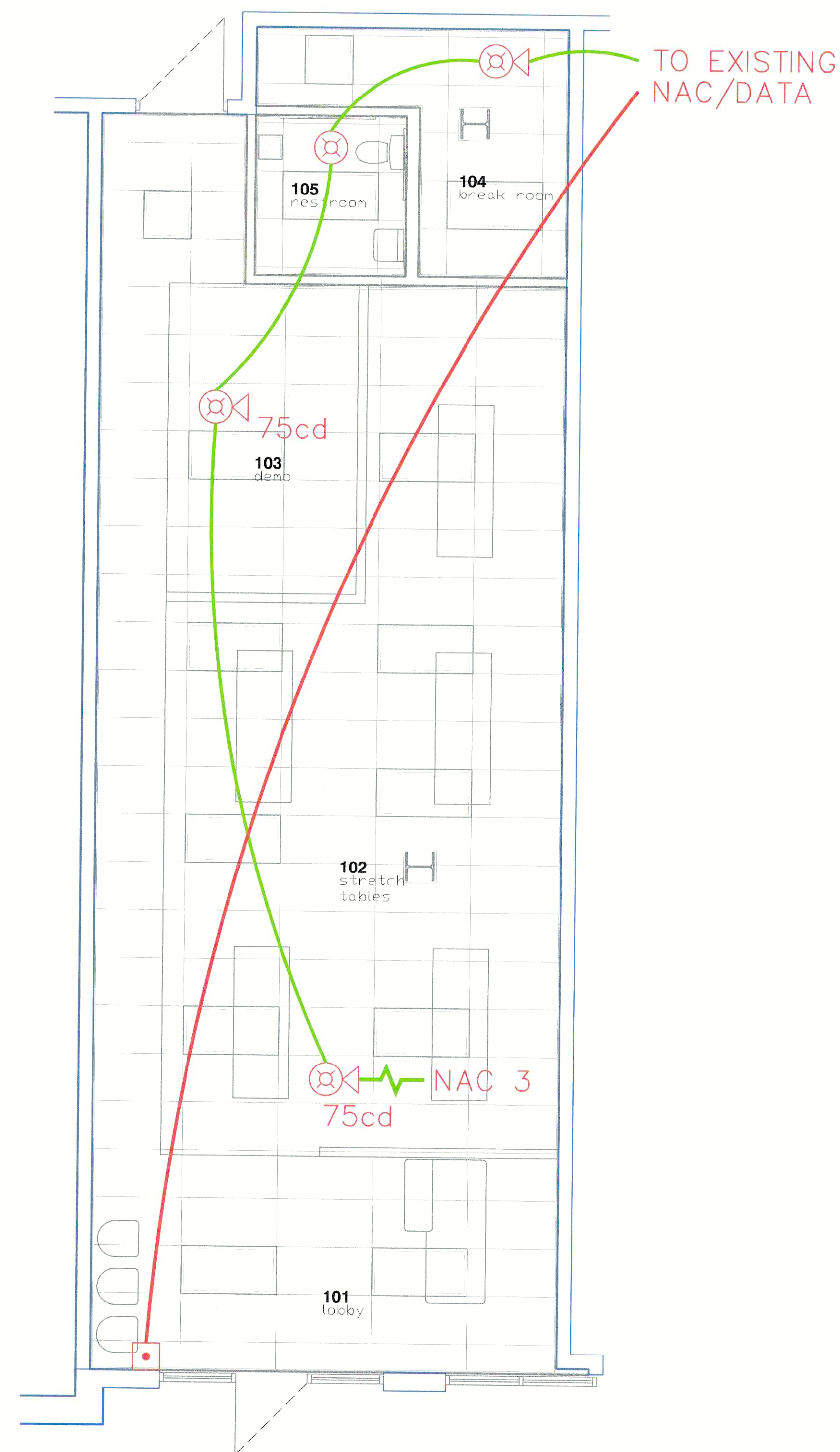
1 FIRE ALARM PLAN 1/4" = 1'0"
