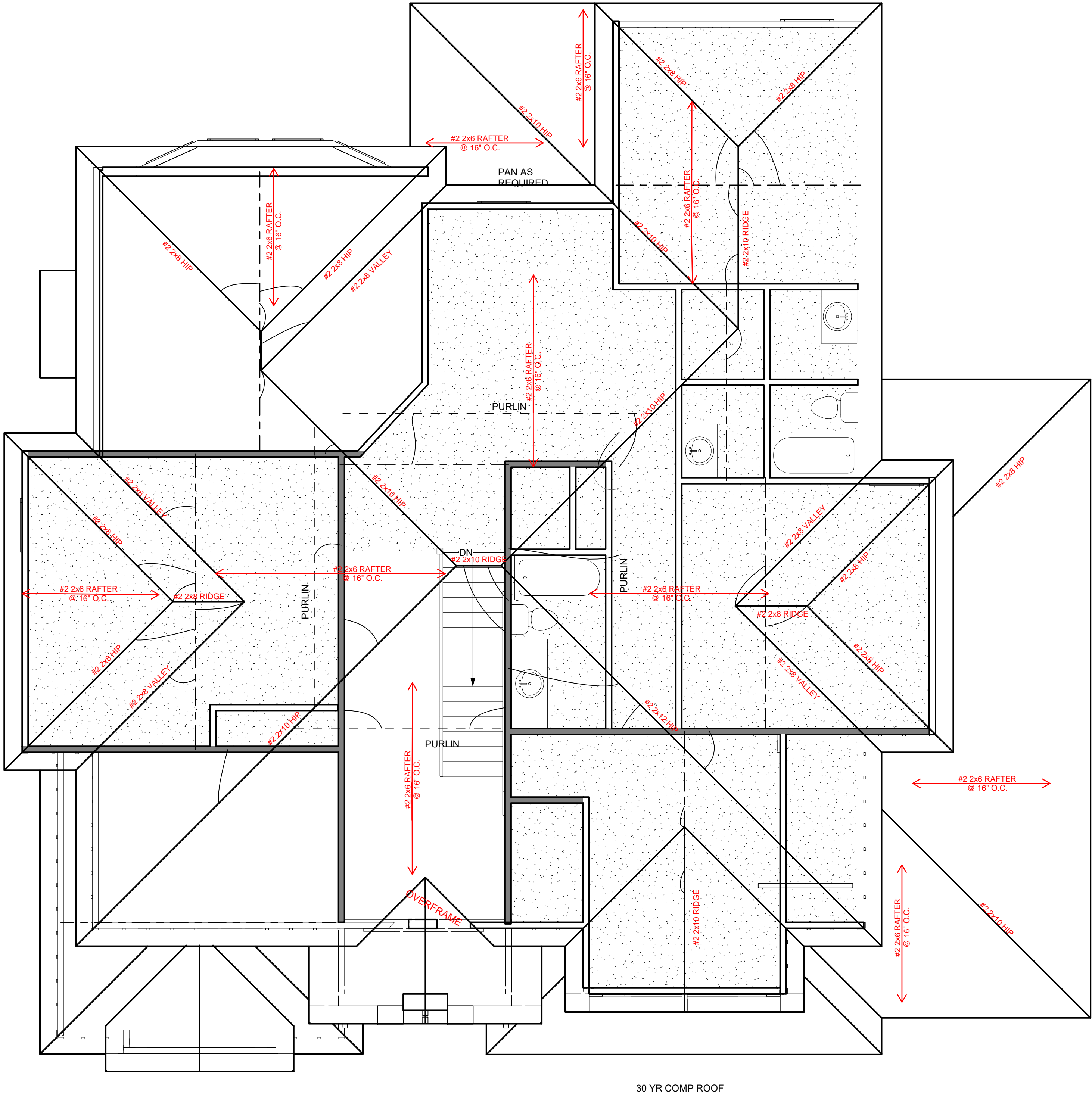
1 ROOF PLAN 1/4" = 1'-0"
