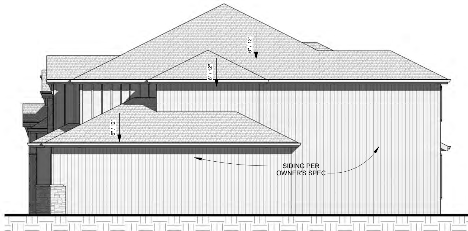
3 RIGHT ELEVATION 1/8" = 1'-0"
