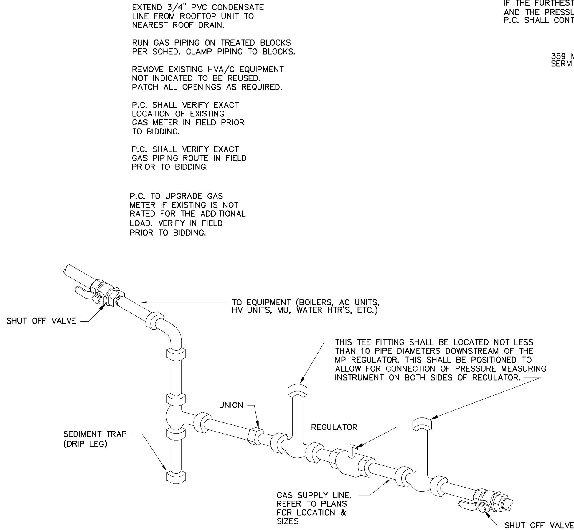
2 TYPICAL GAS PIPING CONNECTION DETAIL FOR THE INSTALLATION OF PRESSURE REGULATORS SCALE: NONE
