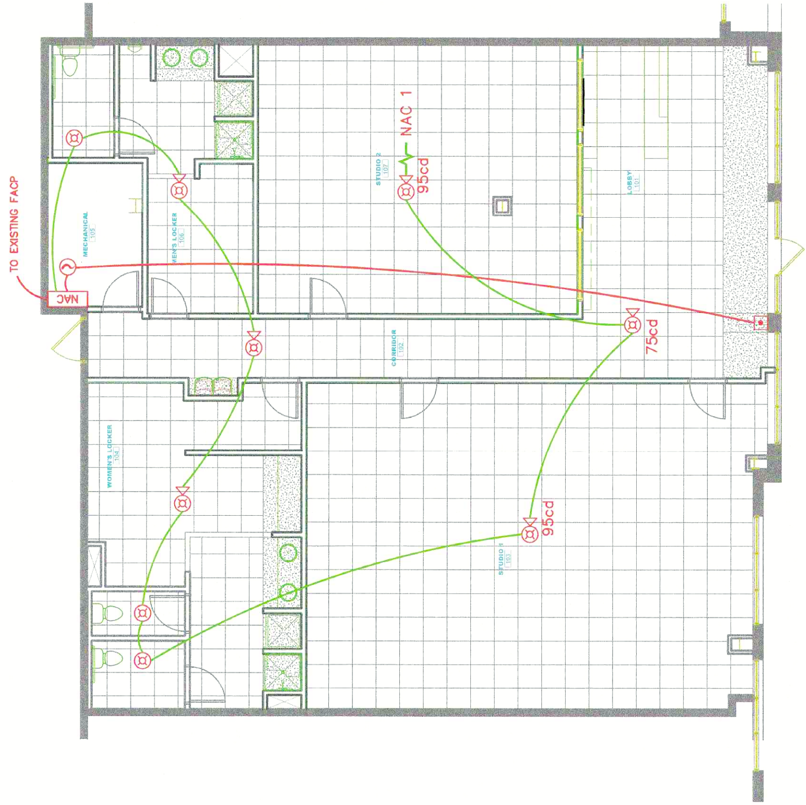
1 FIRE ALARM PLAN 1/8" = 1'0"
