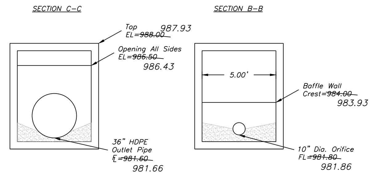
OUTLET STRUCTURE - BASIN E 1" = 1'-0"
