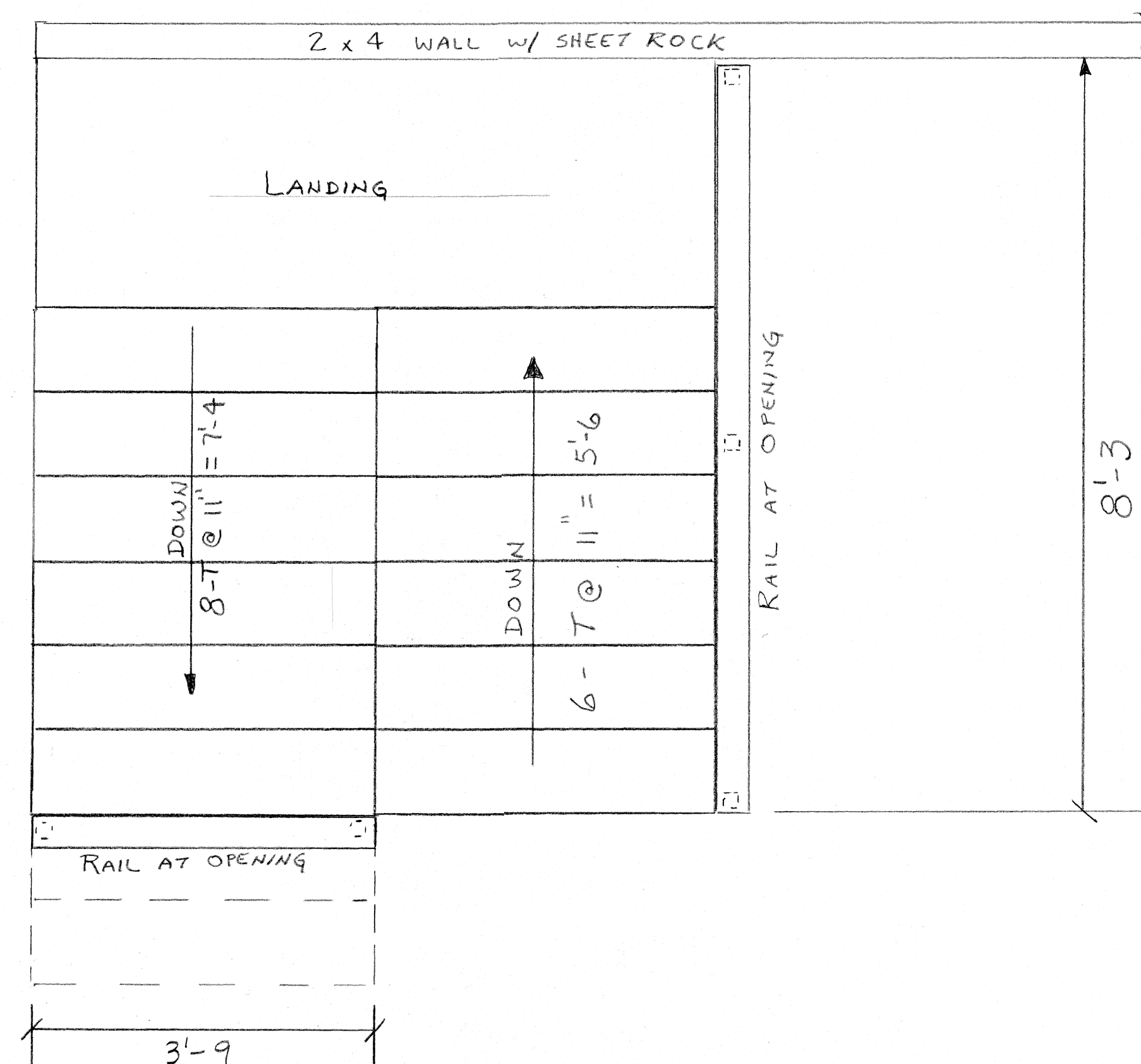
STAIR OPENING PLAN
