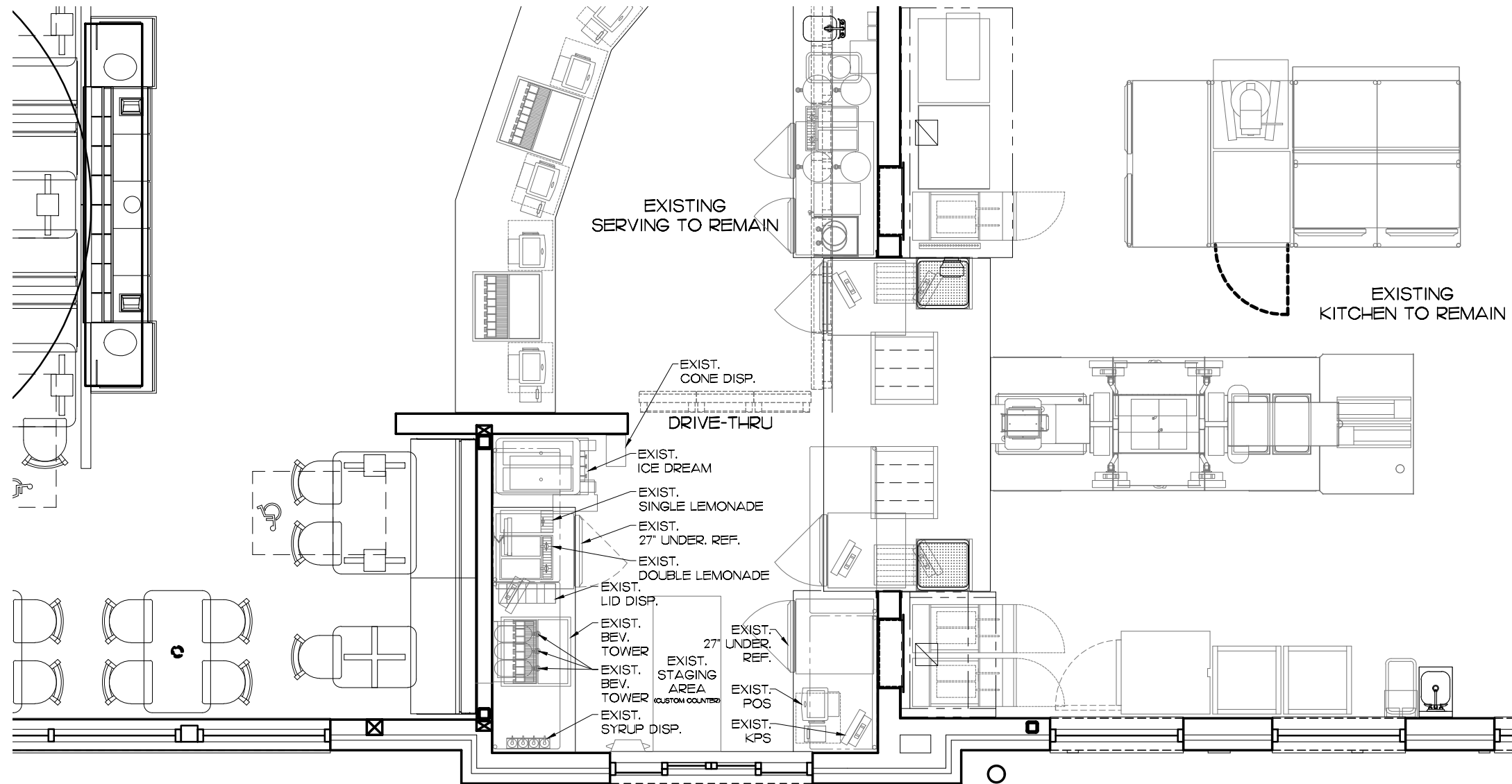
I PARTIAL EQUIPMENT PLAN - SERVING/DRIVE THRU 1/4"=1'-0"
