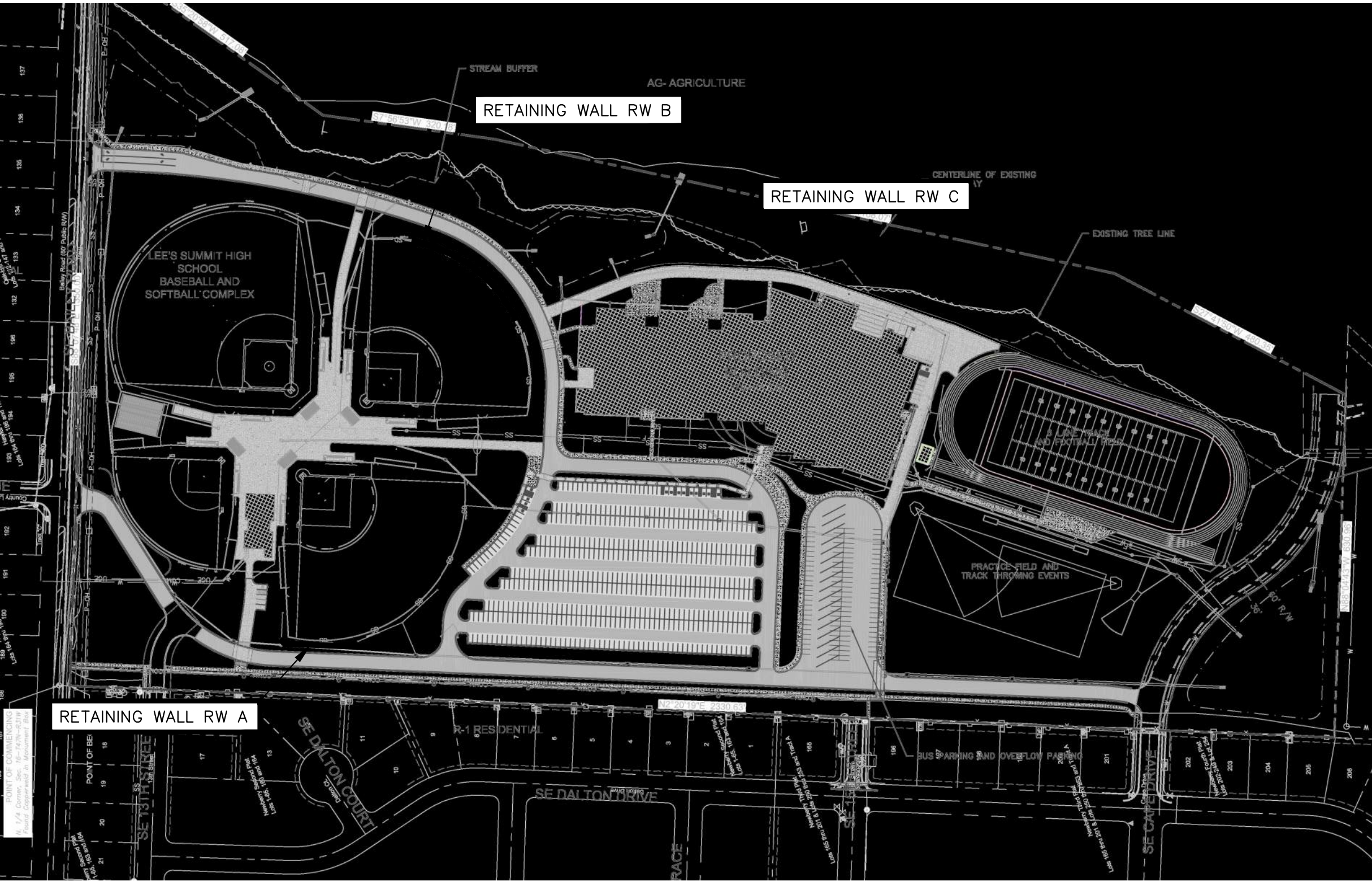
RETAINING WALL - LOCATION MAP
