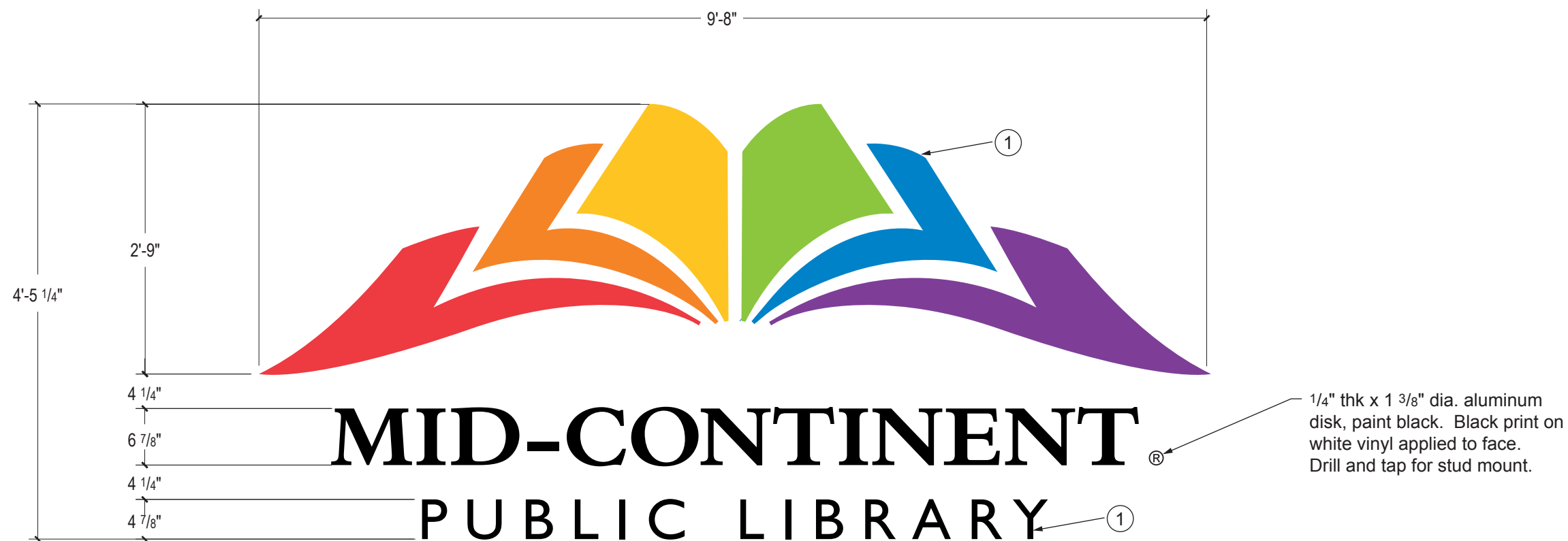
A Logo & Letters, 9'-9" Wide, NON-illuminated scale: 3/4" = 1'-0"
