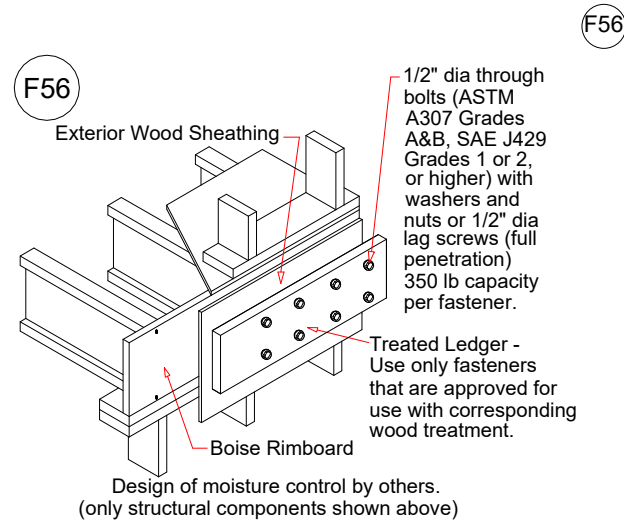
Typical Deck Attachment
