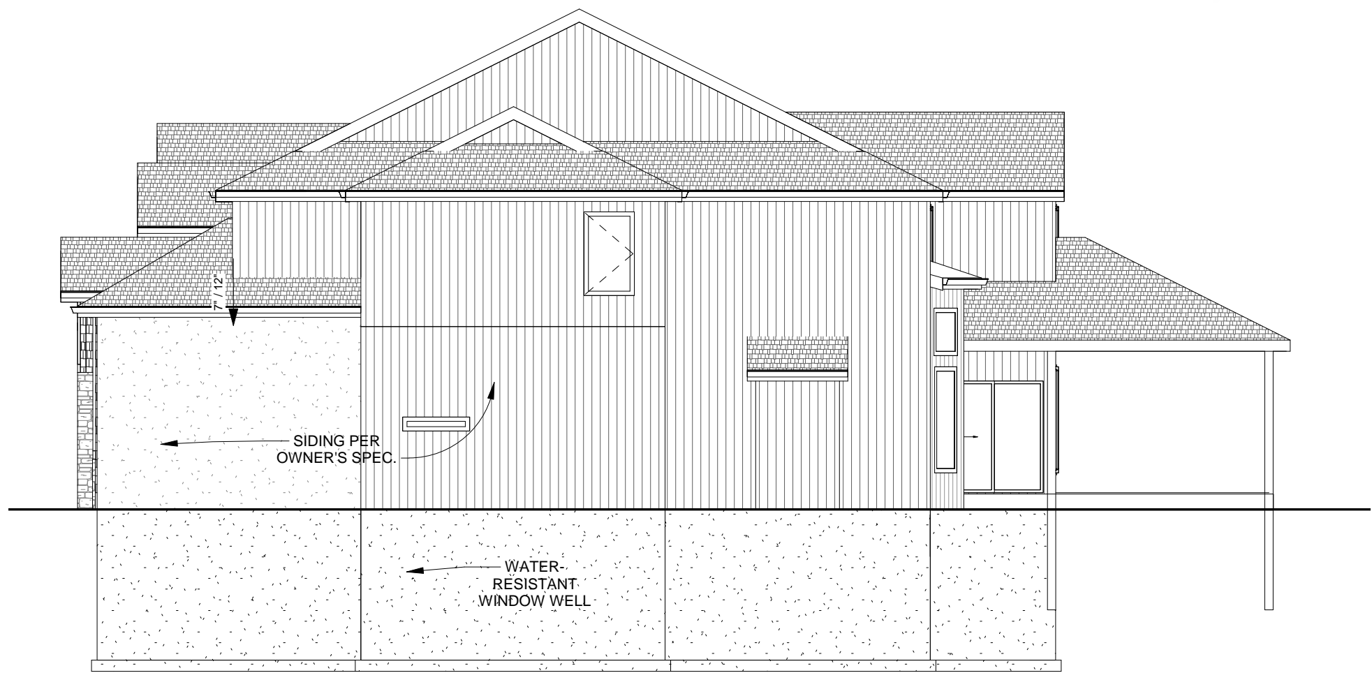
2 LEFT ELEVATION 1/8" = 1'-0"
