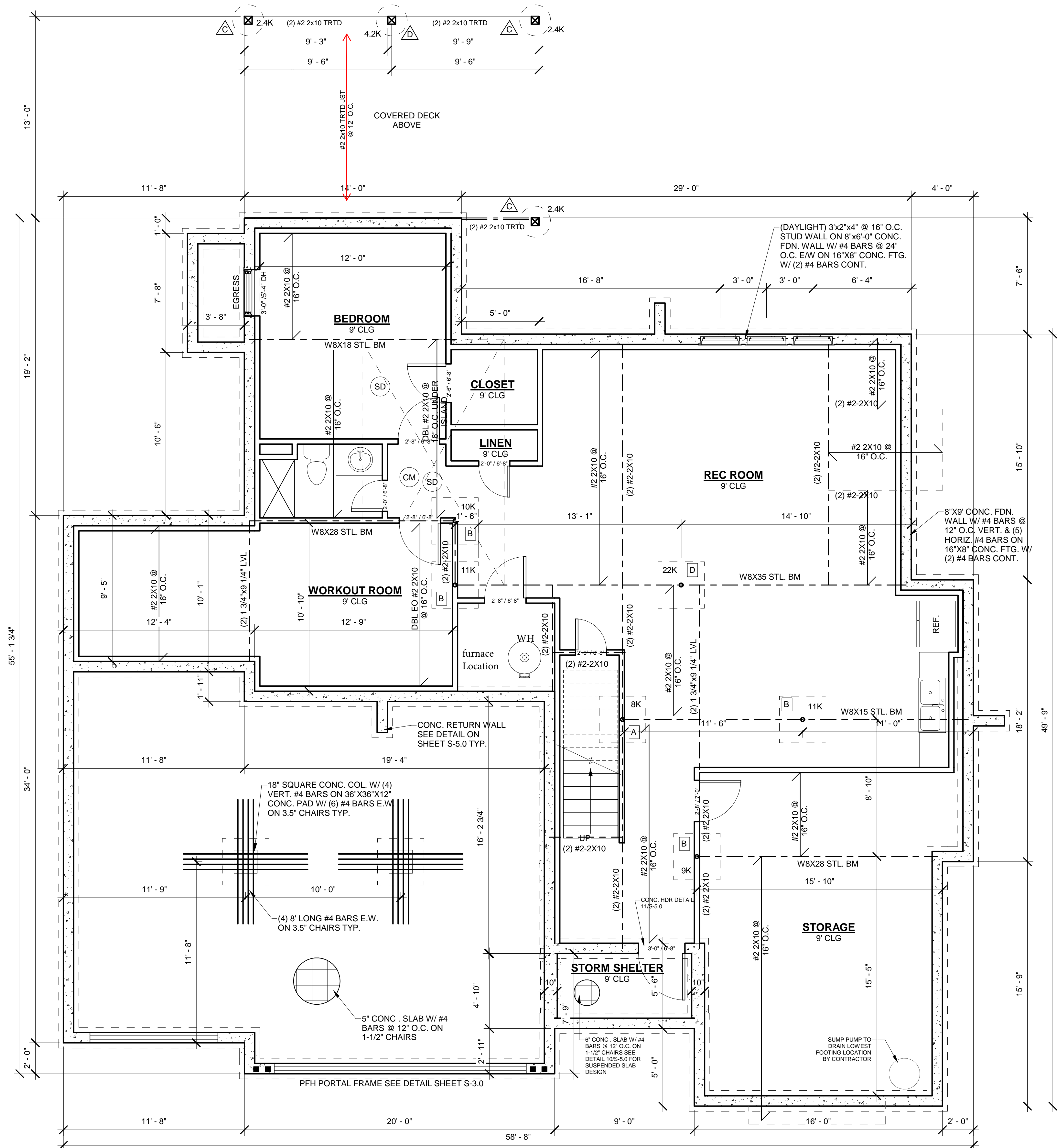
1 FOUNDATION PLAN 1/4" = 1'-0"
