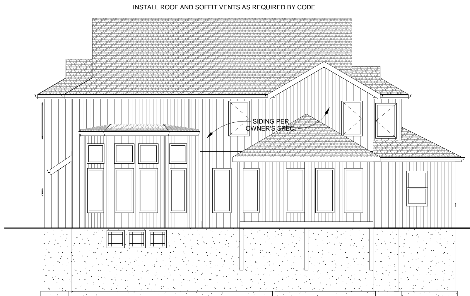
4 REAR ELEVATION 1/8" = 1'-0"
