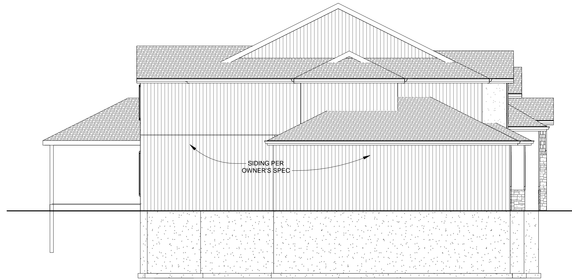
3 RIGHT ELEVATION 1/8" = 1'-0"
