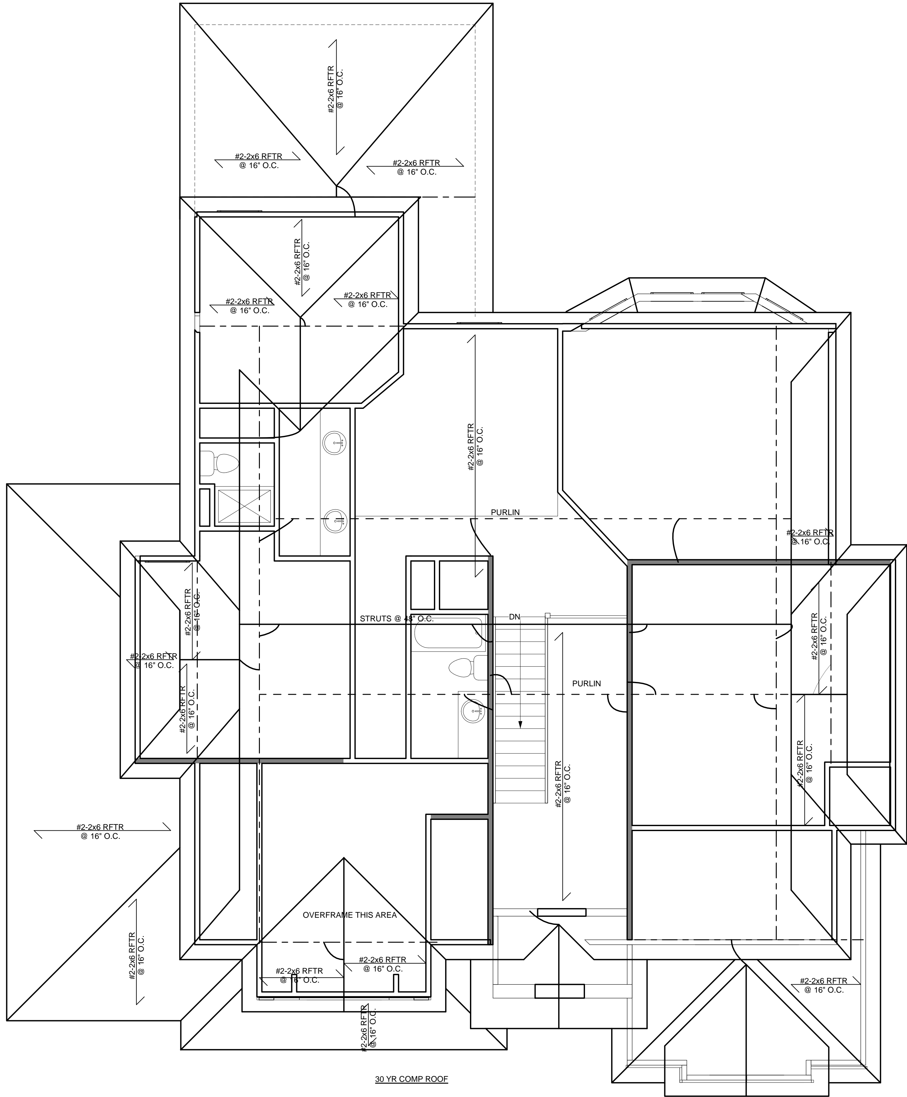
1 ROOF PLAN 1/4" = 1'-0"
