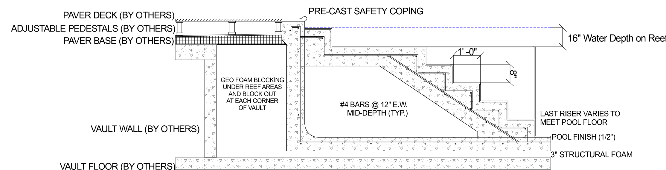
REEF STAIR DETAIL NO SCALE
