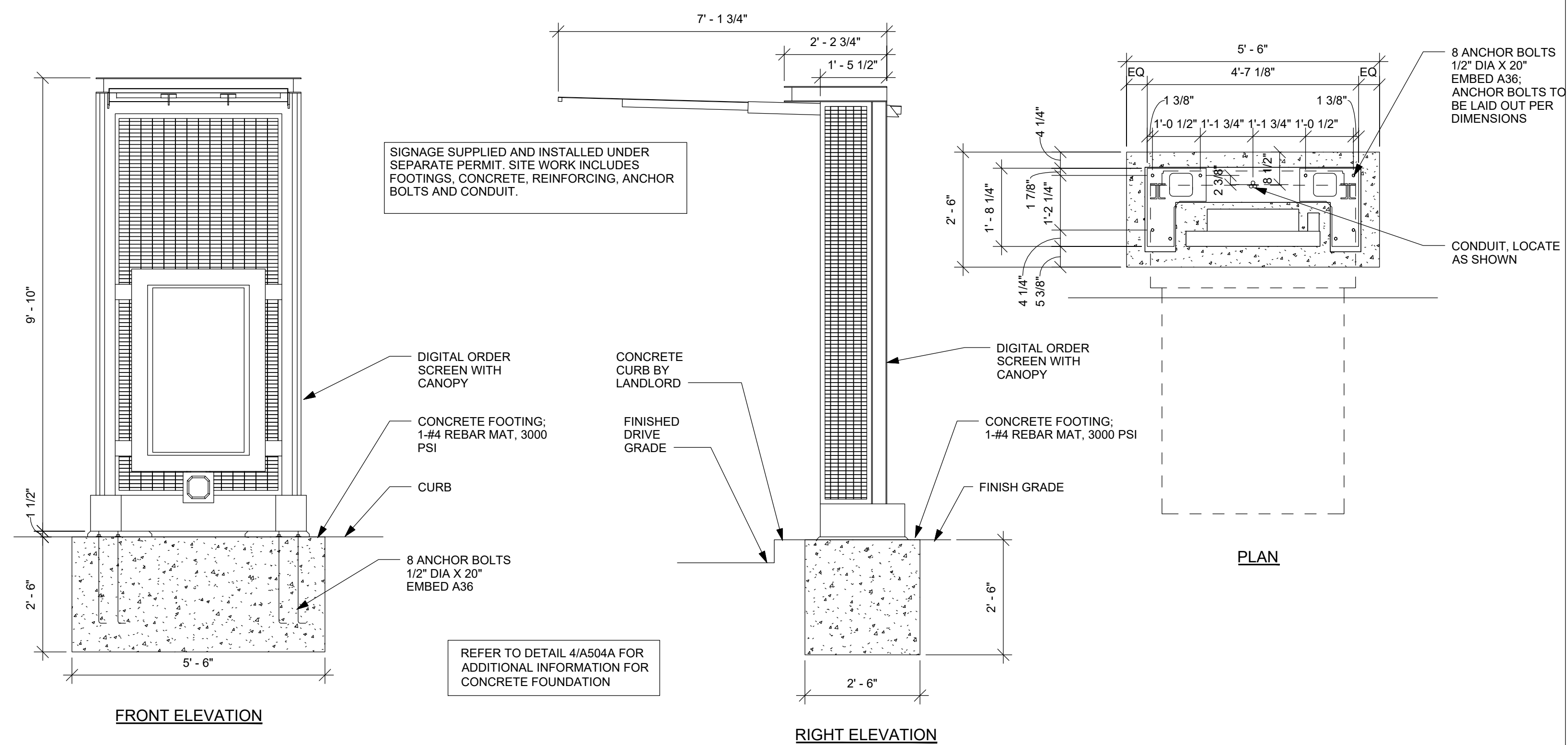
5 DTE - DIGITAL ORDER SCREEN WITH CANOPY A505 SCALE: 1/2" = 1'-0"
