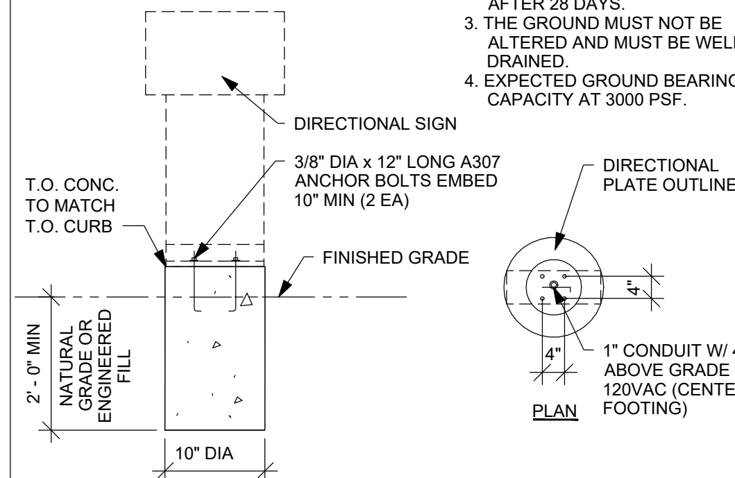
1 DIRECTIONAL SIGNAGE FOOTING A505 SCALE: 1/2" = 1'-0"
