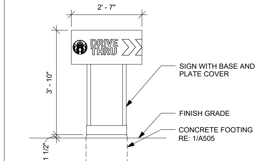
3 DTE - DIRECTIONAL SIGN WITH (ENTRY) A505 SCALE: 1/2" = 1'-0"
