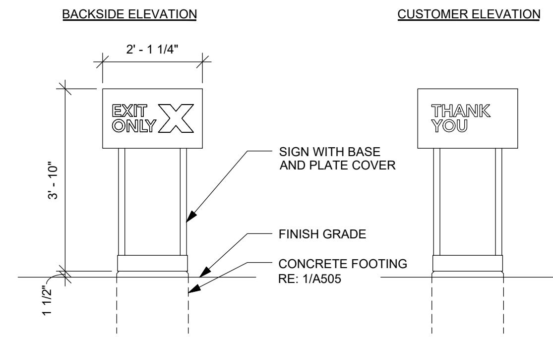
2 DTE - DIRECTIONAL SIGN (EXIT) A505 SCALE: 1/2" = 1'-0"
