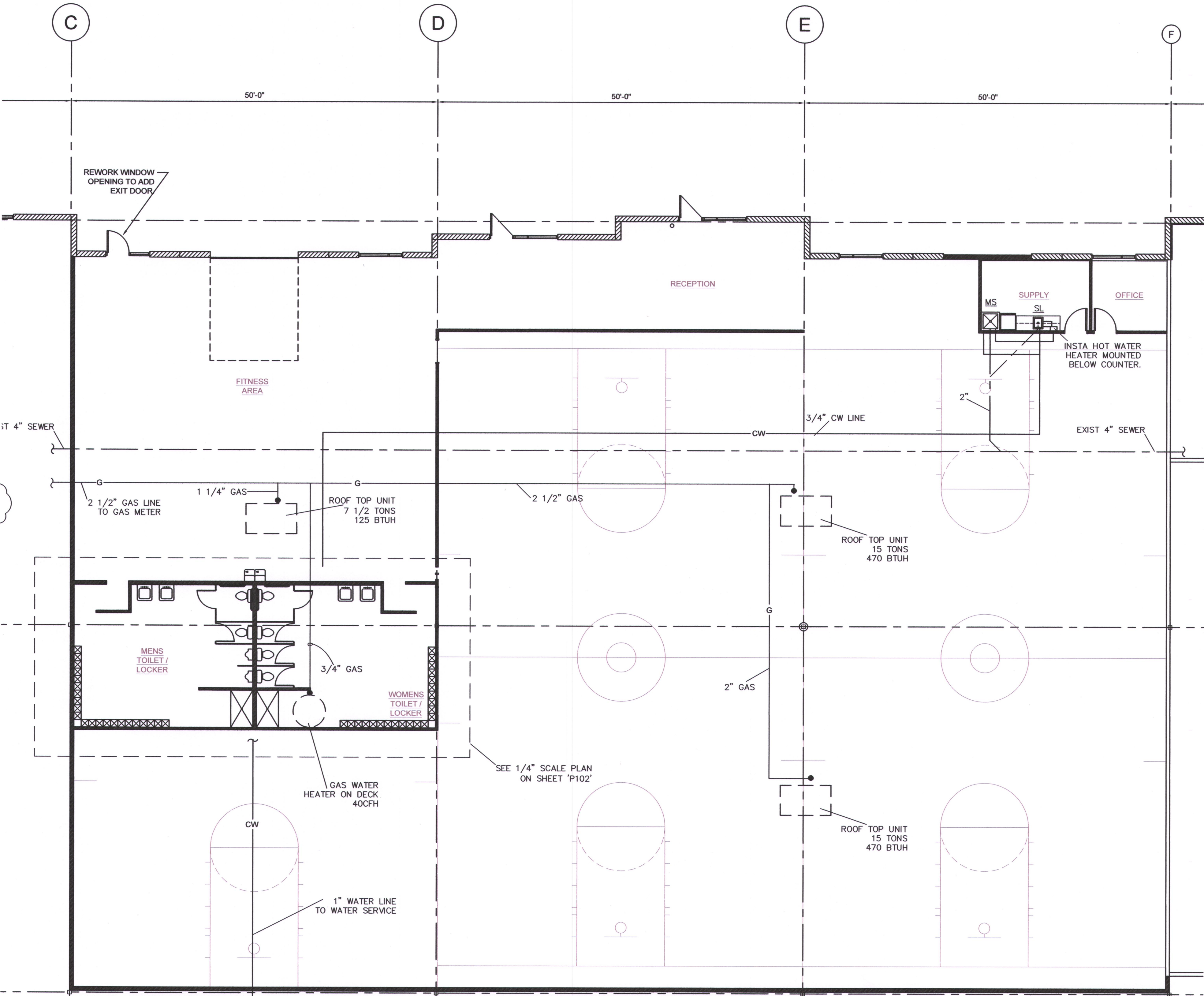
1 Floor Plan scale: 1/8"=1'-0"
