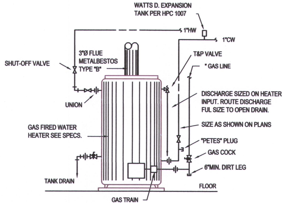
GAS WATER HEATER DETAIL NO SCALE APPROX. 1000 LBS OPERATING WEIGHT
