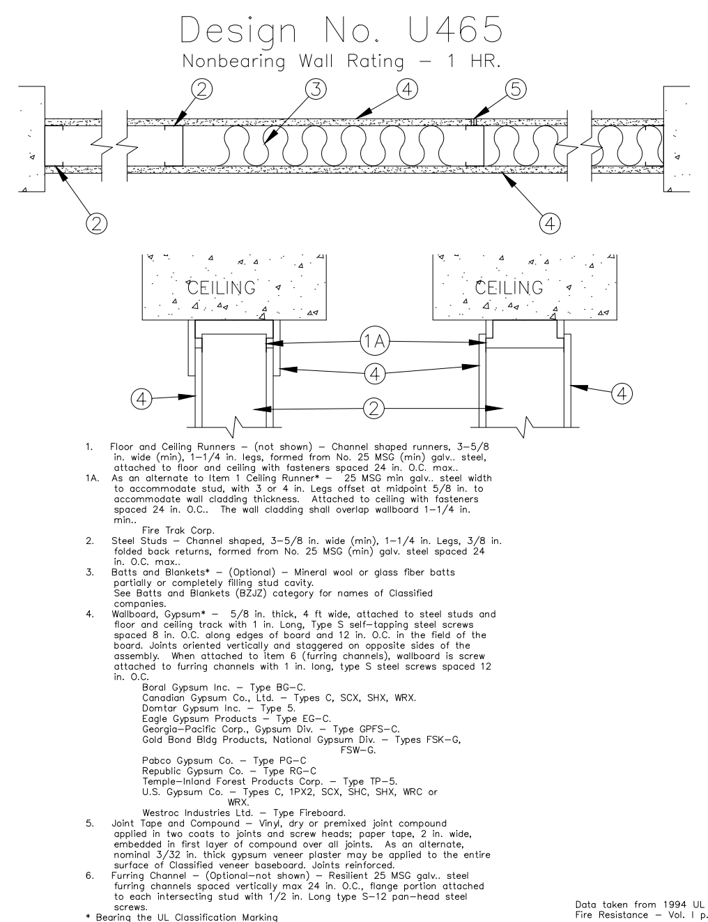
5 FIRE-RATED ASSEMBLY scale: None
