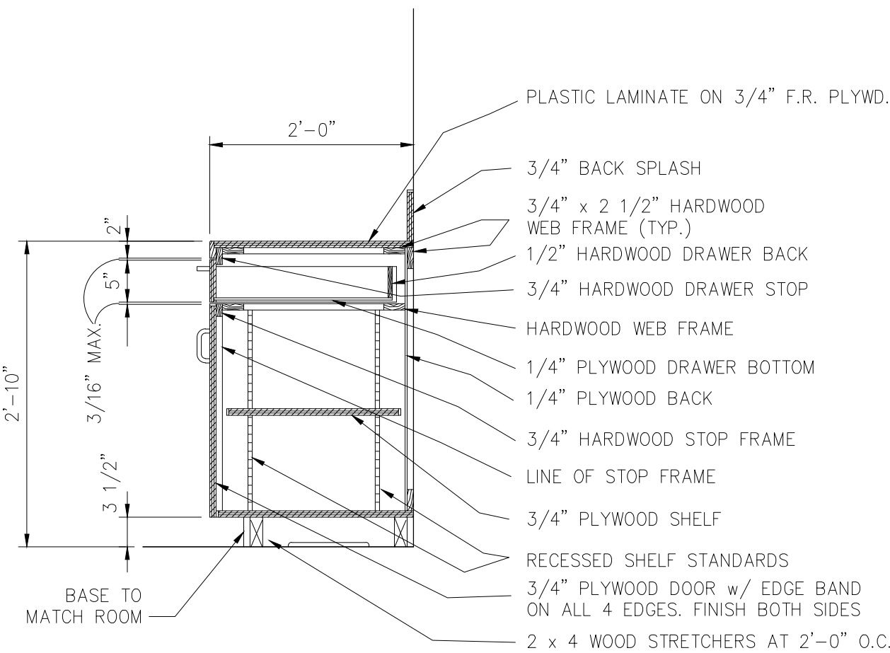
6 COUNTER SECTION scale: 1/2=1'-0"
