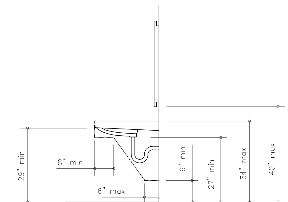
2 LAVATORY CLEARANCES scale: 1/2=1'-0"
