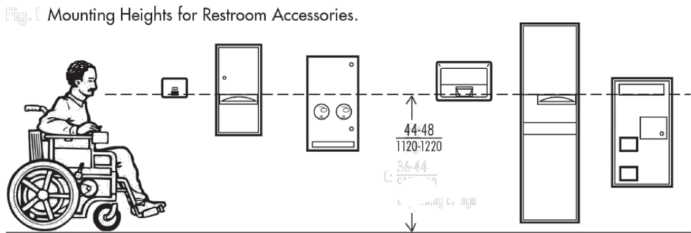
3 ACCESSORY MOUNTING HEIGHTS scale: None
