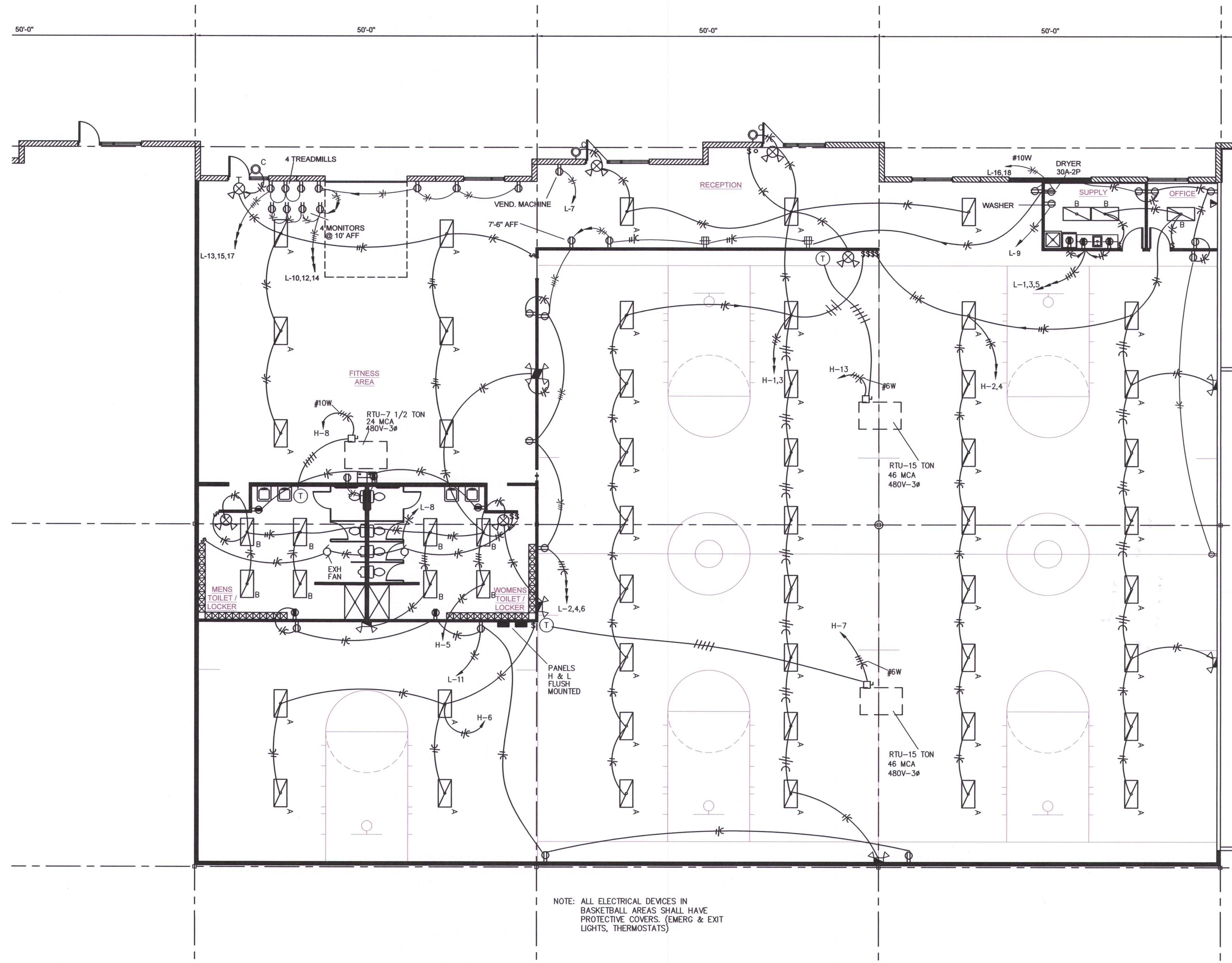
1 Floor Plan scale: 1/8"=1'-0"
