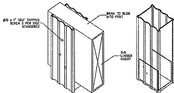
POST/BEAM CONNECTION
