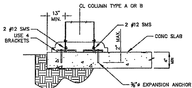
COLUMN TO SLAB DETAIL (B4) (ATTACHED TO HOUSE)
