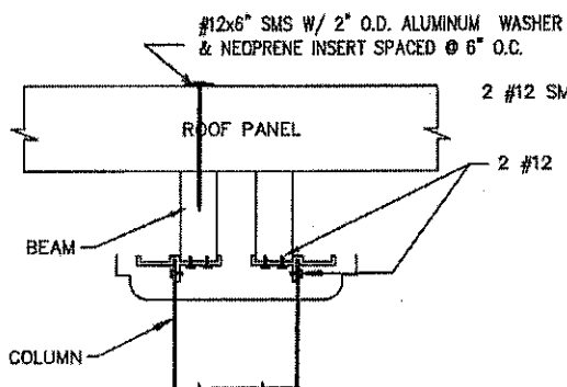
ROOF PANEL/DOUBLE BEAM/COLUMN CONNECTION (B5)
