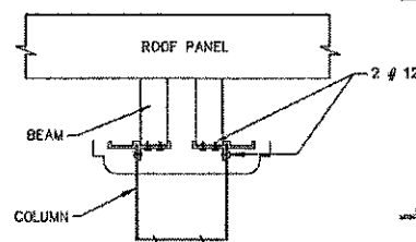
DOUBLE BEAM/COLUMN CONNECTION
