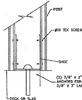
SLAB CONNECTION SIDE VIEW
