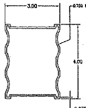
PATIO POST (16543) (31)
