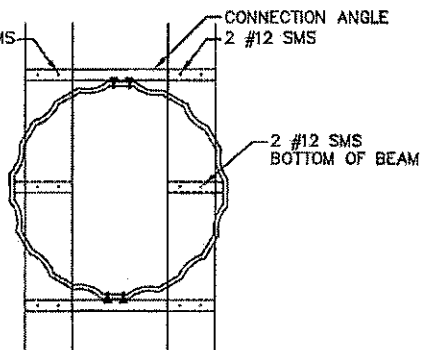
ROOF PANEL/DOUBLE BEAM/COLUMN CONNECTION (B5)
