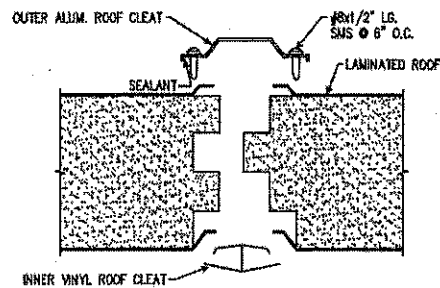
ROOF PANEL SPLICE (B1)
