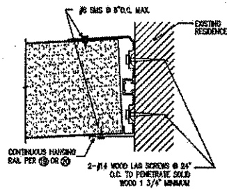
ROOF PANEL/WALL ATTACHMENT (B2)
