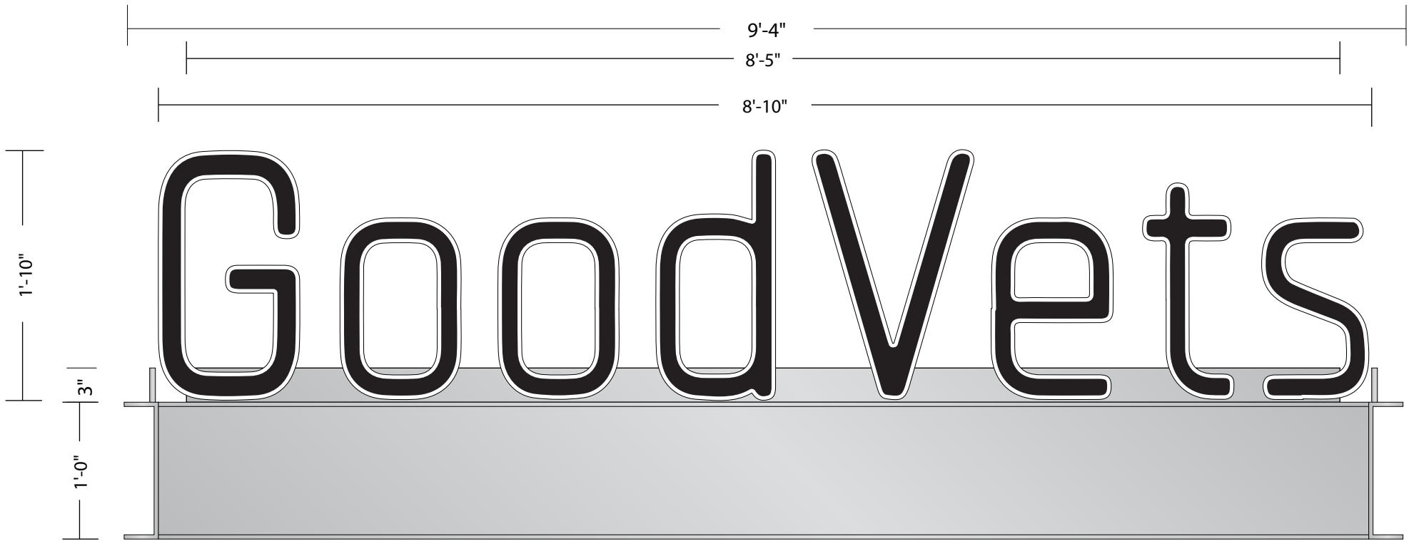
Front View 1" = 1'-0"
