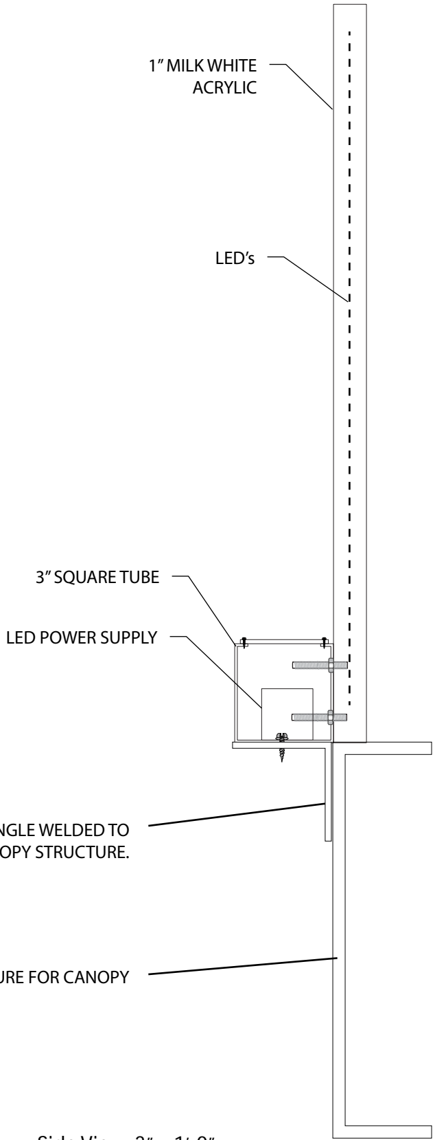
Side View 3" = 1'-0"
