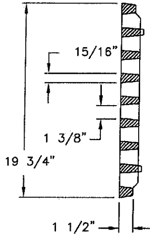
GRATE SECTION
