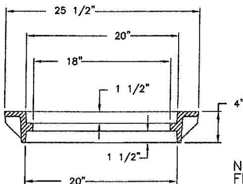
FRAME SECTION
