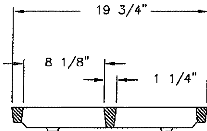
GRATE SECTION
