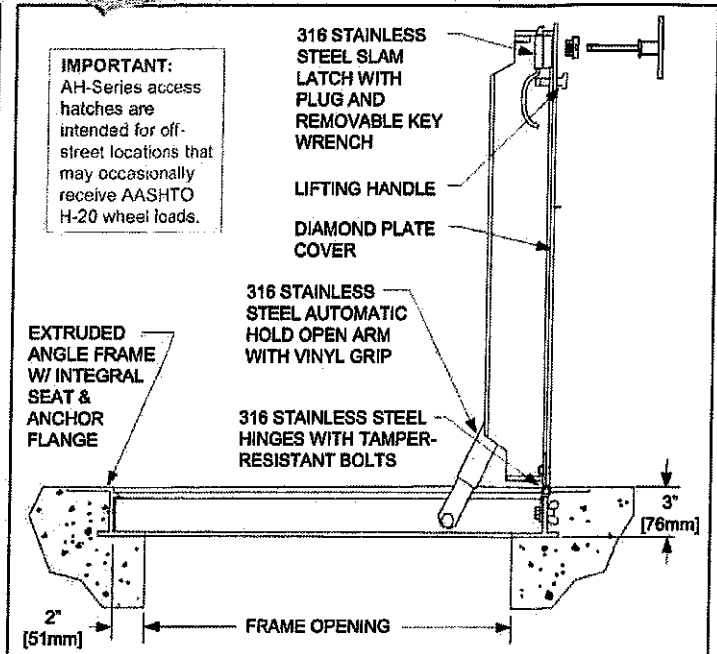
Model AHS & AHD H-20 Vehicle Load Rating
