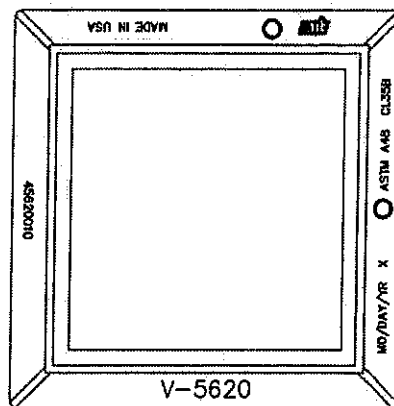
FRAME BOTTOM FLANGE VIEW
