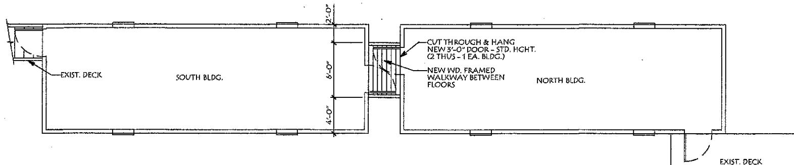
EXIST. FLOOR PLANS
