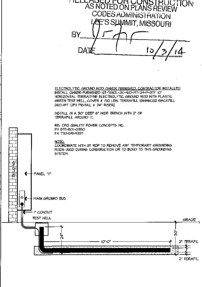
A13 ELECTROLYTIC GROUND ROD NOT TO SCALE
