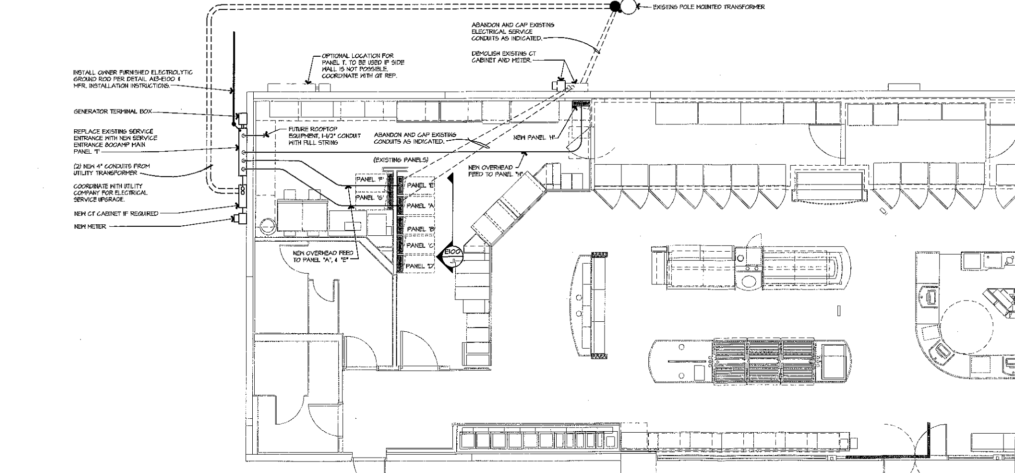
A1 ELECTRICAL FLOOR PLAN 1/4" = 1'-0"
