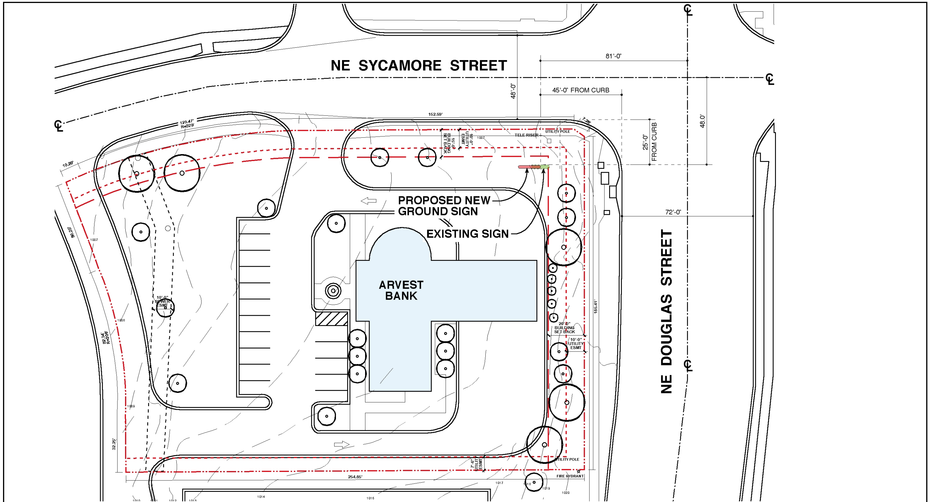
1 SITE PLAN SCALE : 3/8" = 12'-0" -LOCATION OF GROUND SIGN ON PROPERTY
