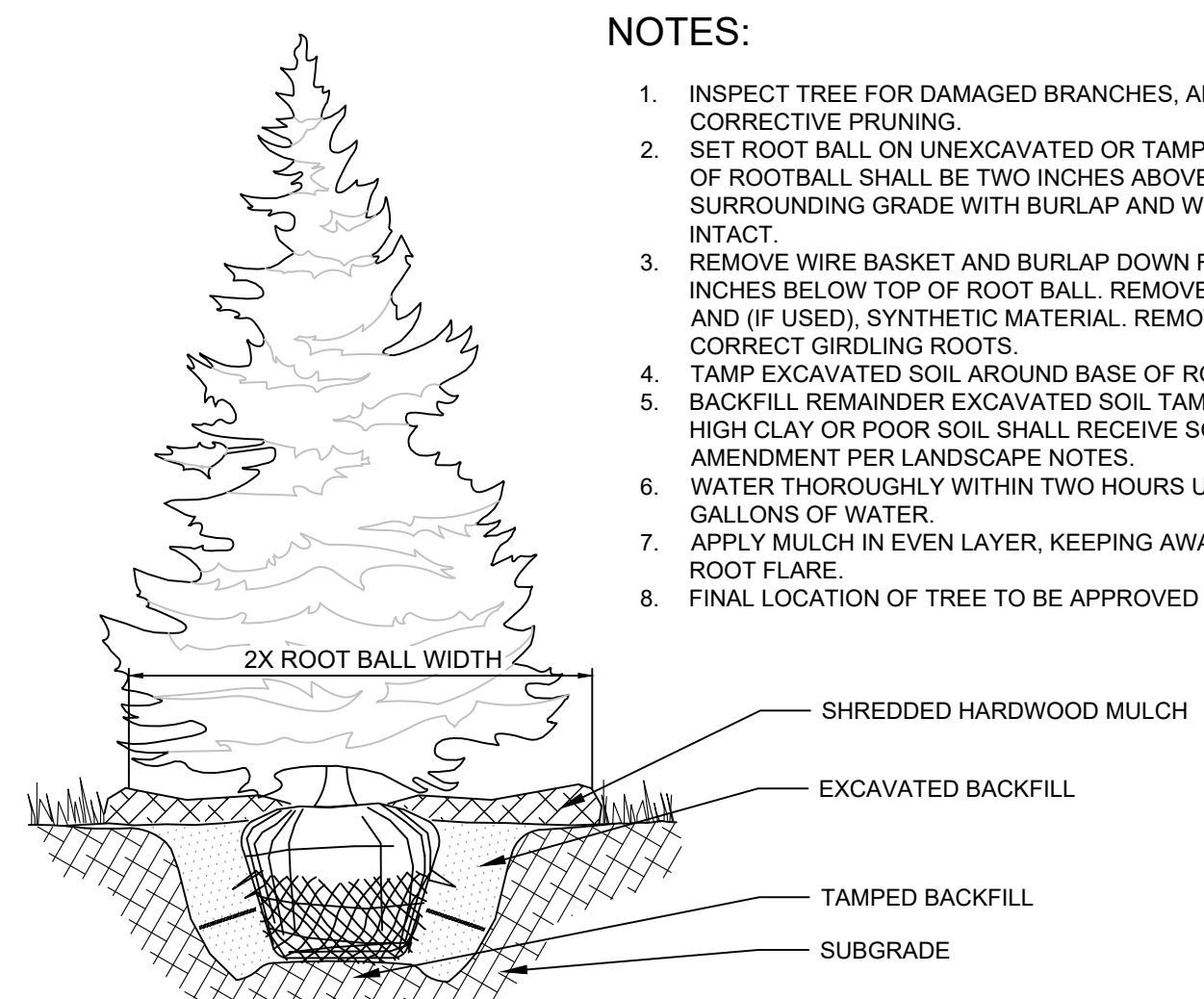
3 EVERGREEN TREE PLANTING NTS
