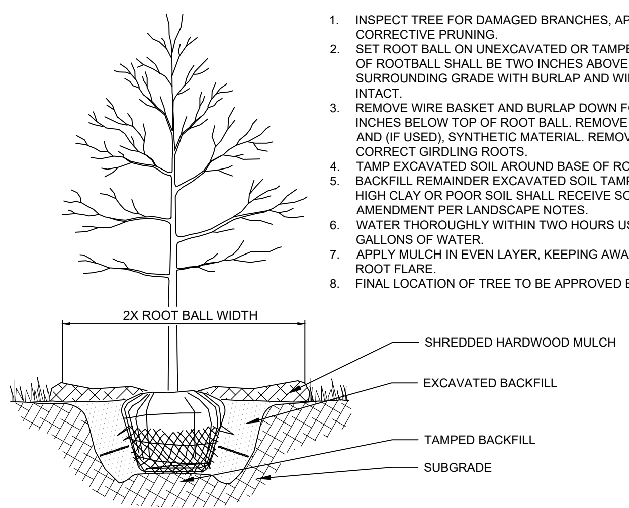
1 TREE PLANTING NTS
