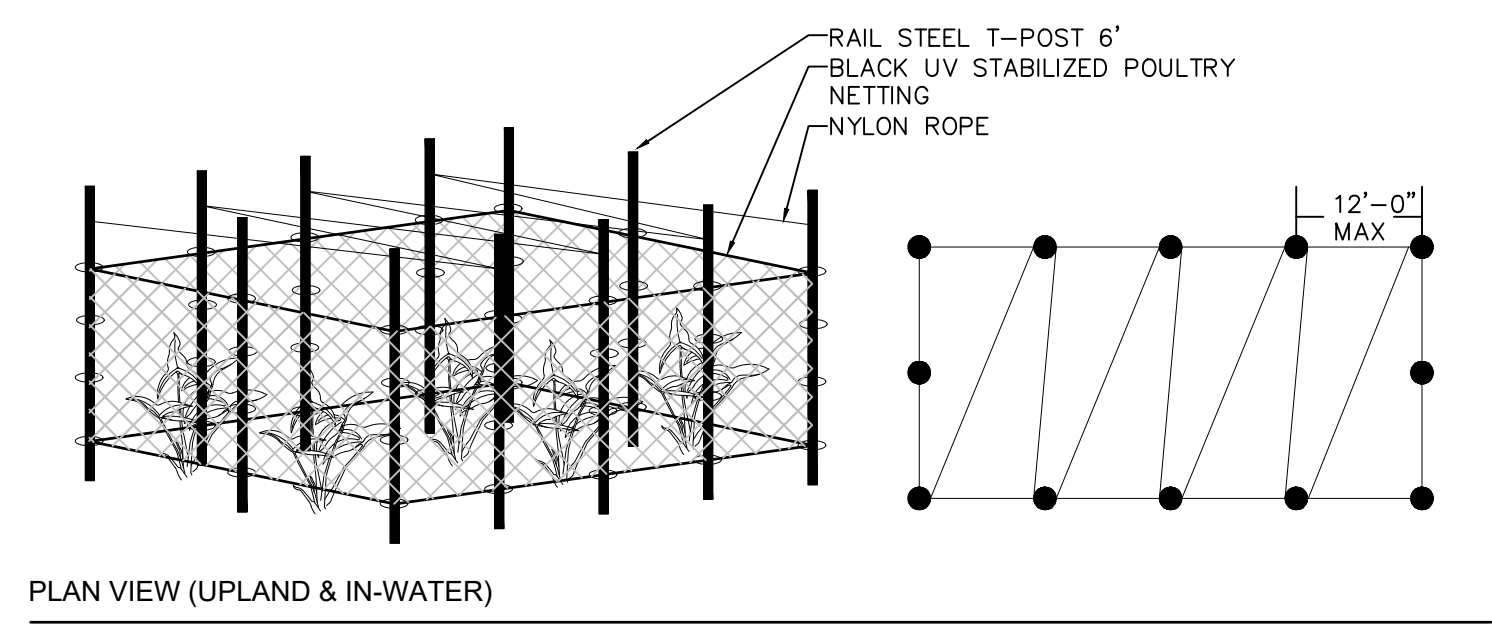
8 GOOSE ENCLOSURE FENCING 1" = 1'-0"
