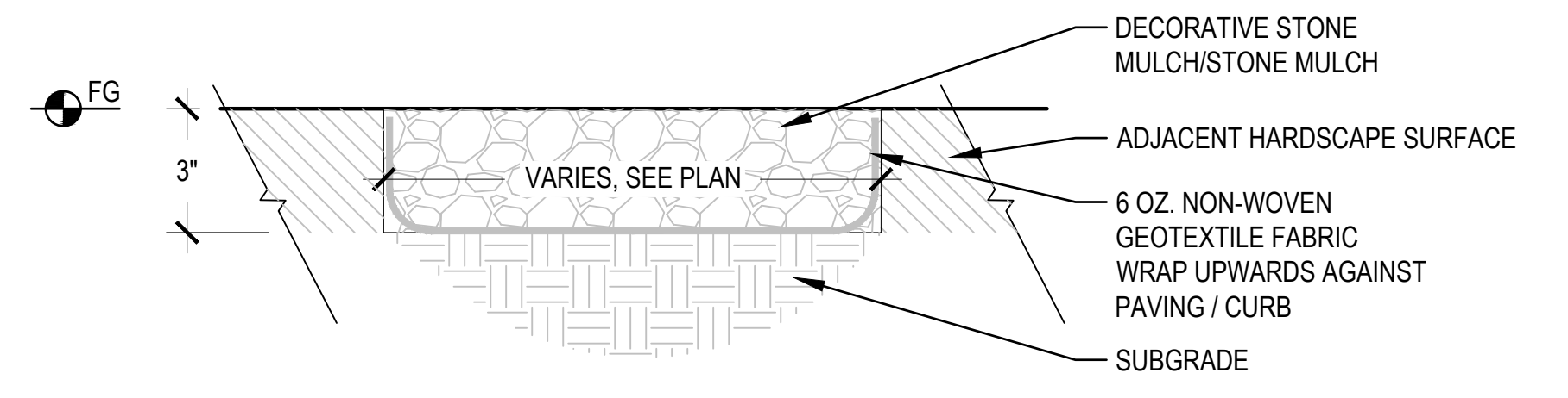
9 STONE MULCH ADJACENT TO HARDSCAPE 3" = 1'-0"
