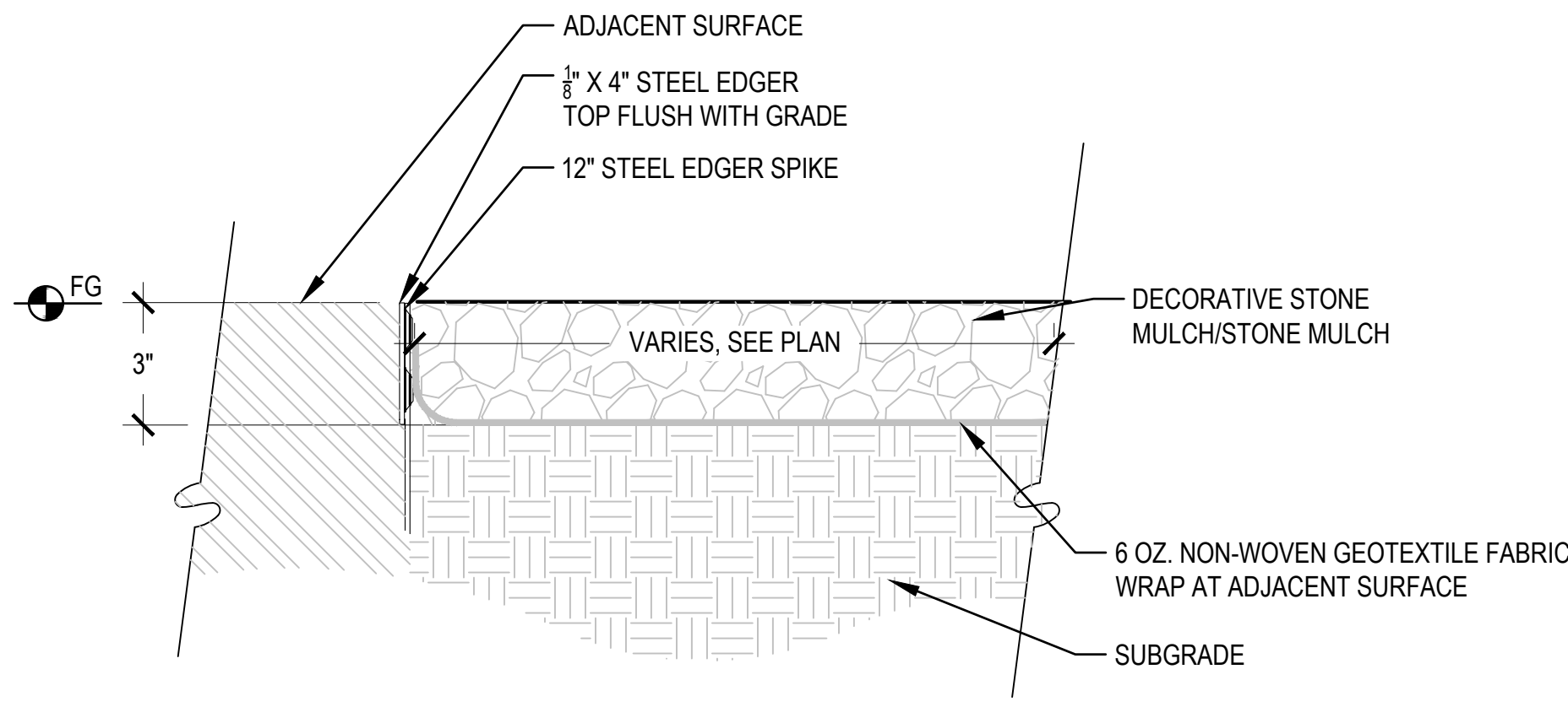
6 STONE MULCH 3" = 1'-0"
