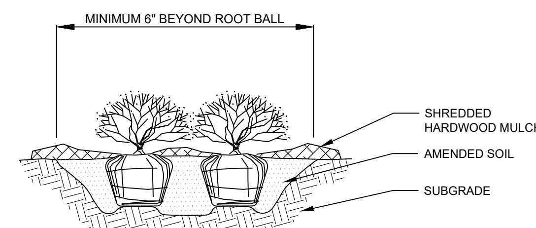
1 TREE PLANTING NTS
