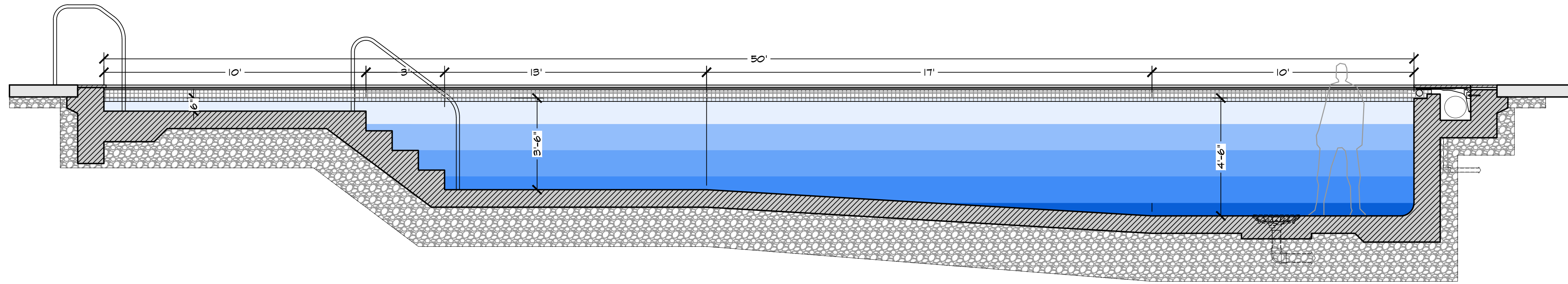
1 POOL CROSS SECTION SCALE: 3/8" = 1'-0" SECTION
