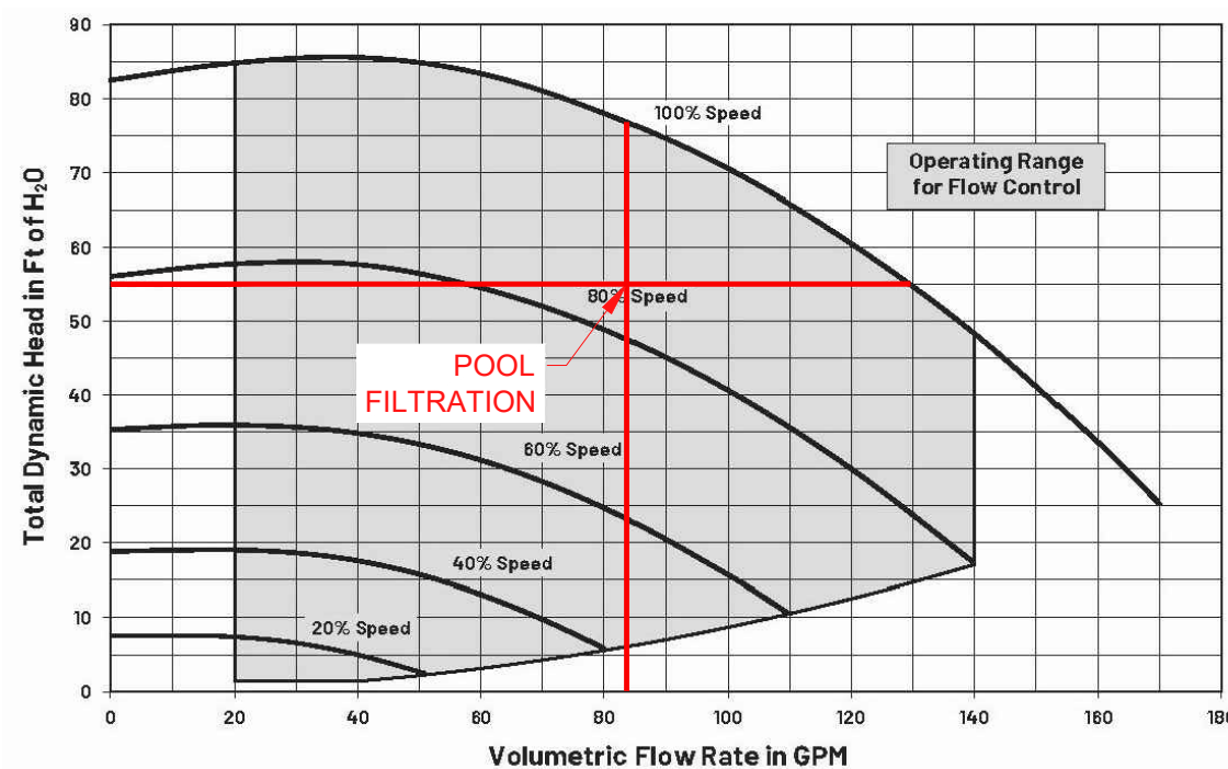
1 PENTAIR INTELLIFLO 3 3HP PUMP SCALE: NTS FILTRATION PUMP CURVE
