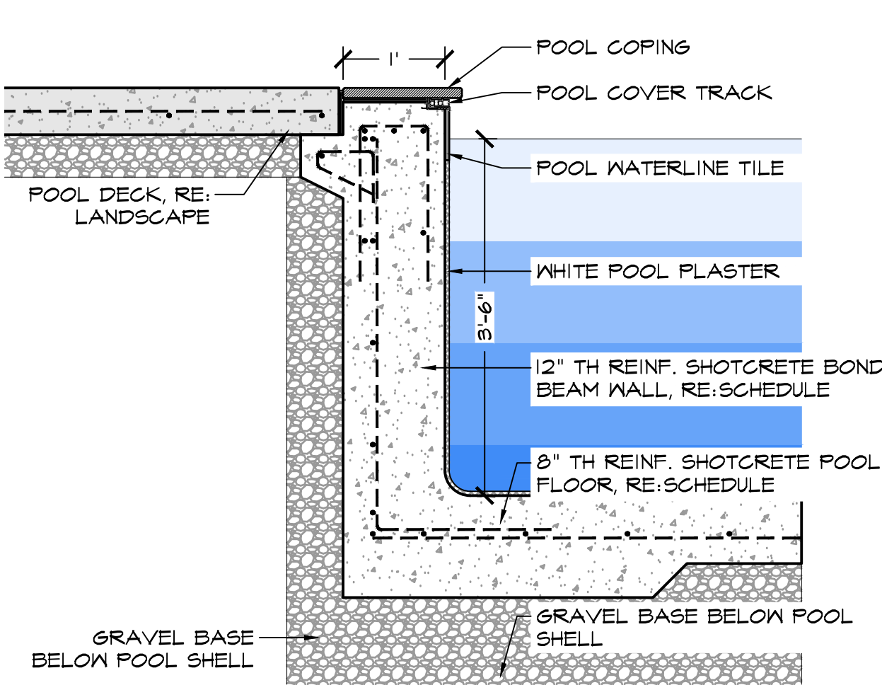
5 SHALLOW END SCALE: 3/4" = 1'-0" SECTION
