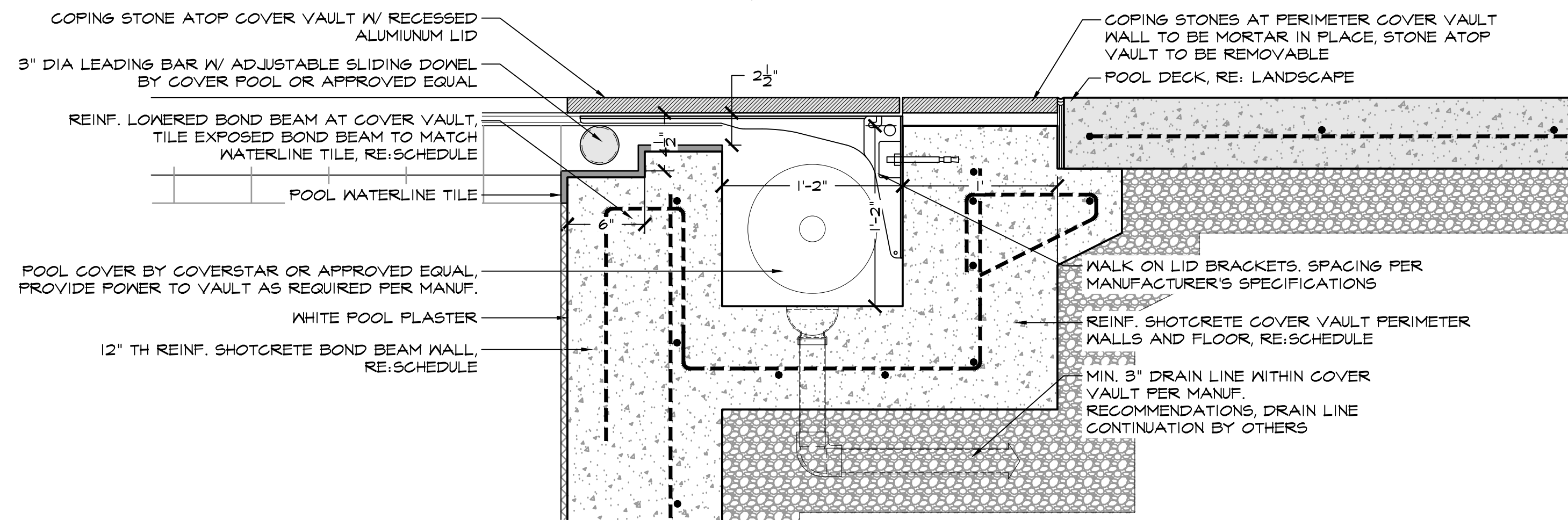
7 POOL COVER VAULT SCALE: 1-1/2" = 1'-0" SECTION
