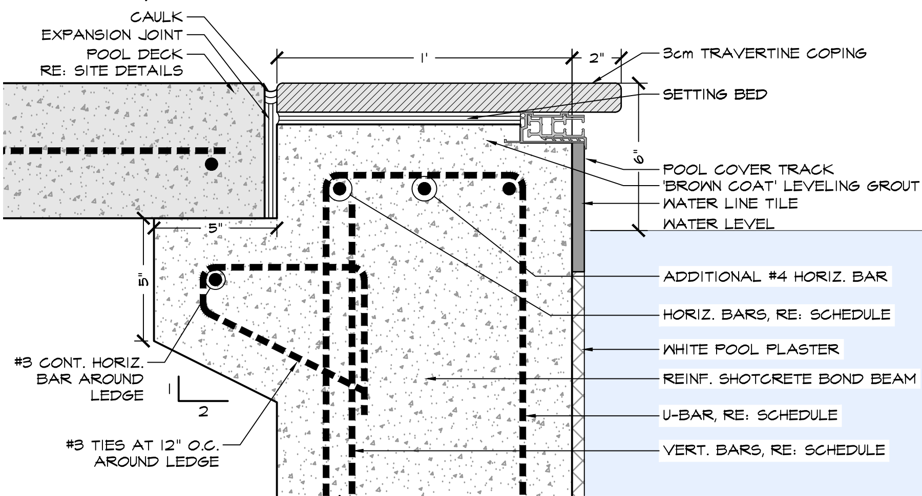
2 TYP. BOND BEAM AND COPING SCALE: 3" = 1'-0" SECTION
