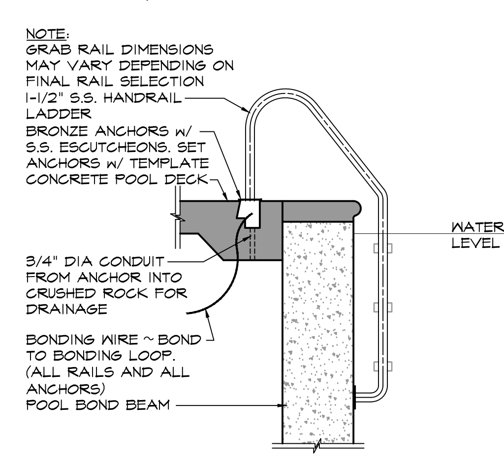
9 LADDER DETAIL SCALE: 3/4" = 1'-0" SECTION
