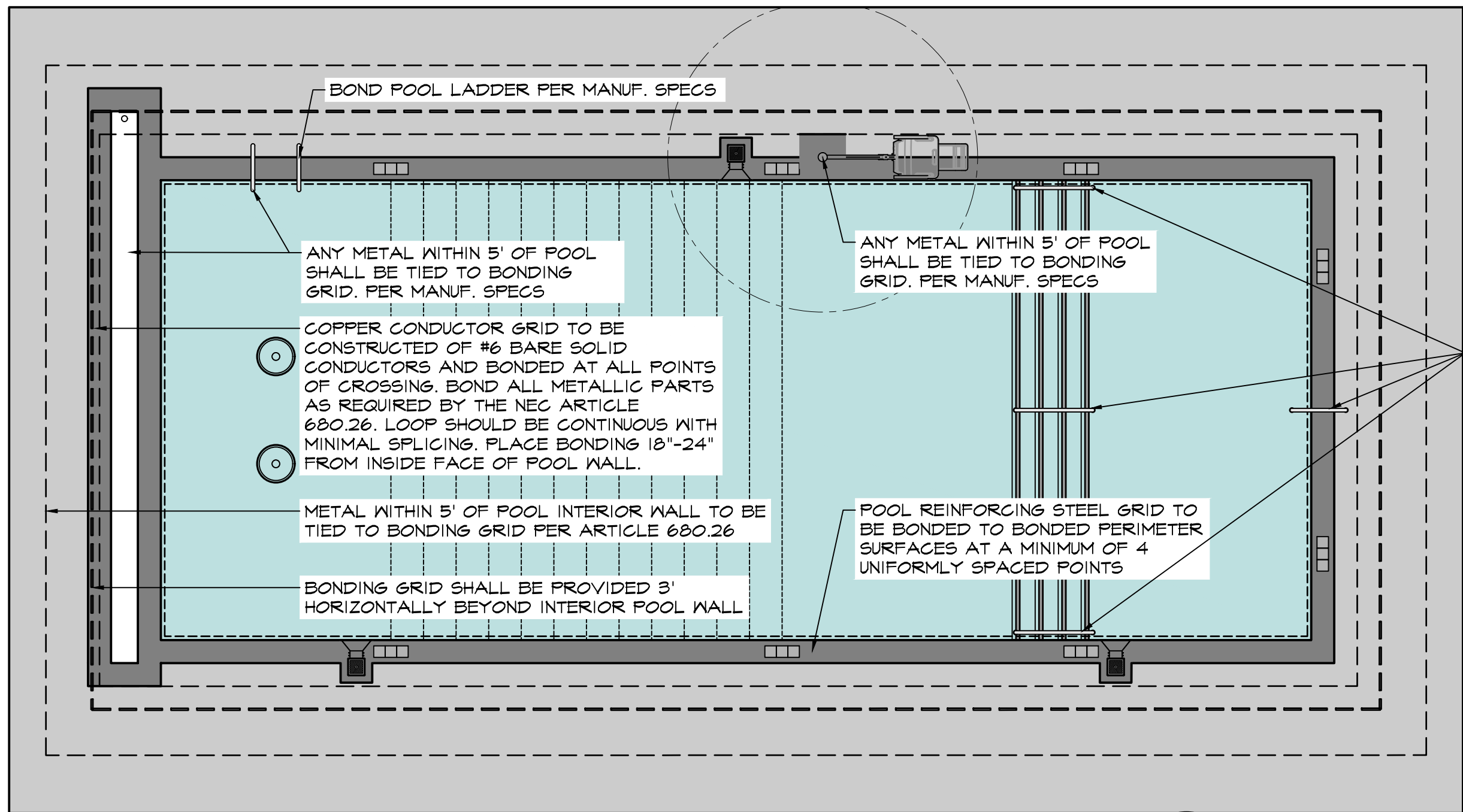
POOL BONDING PLAN SCALE: 1" = 5'-0"
