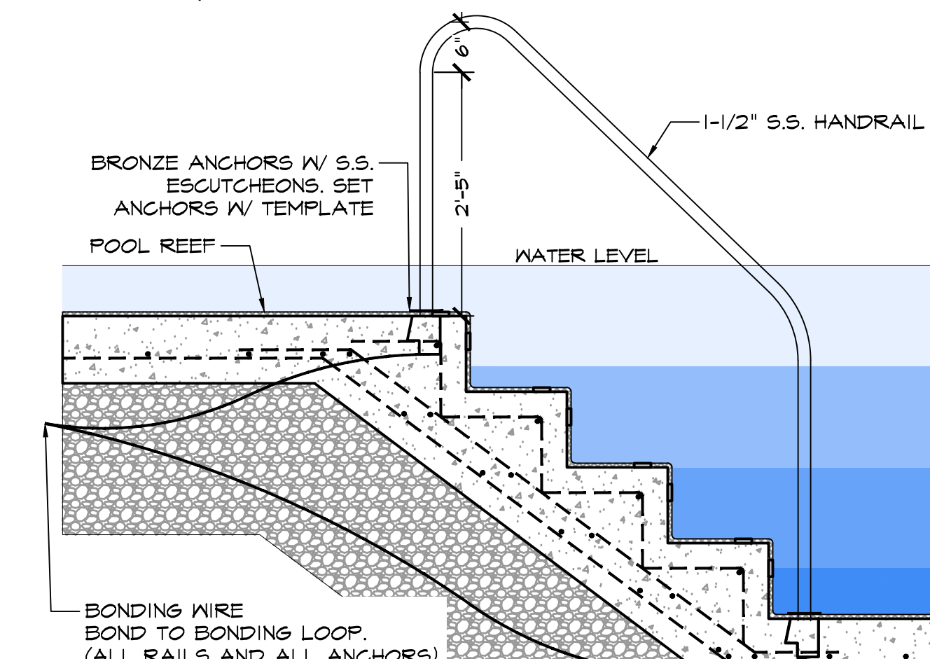
8 REEF HANDRAIL SCALE: 1" = 20'-0" SECTION
