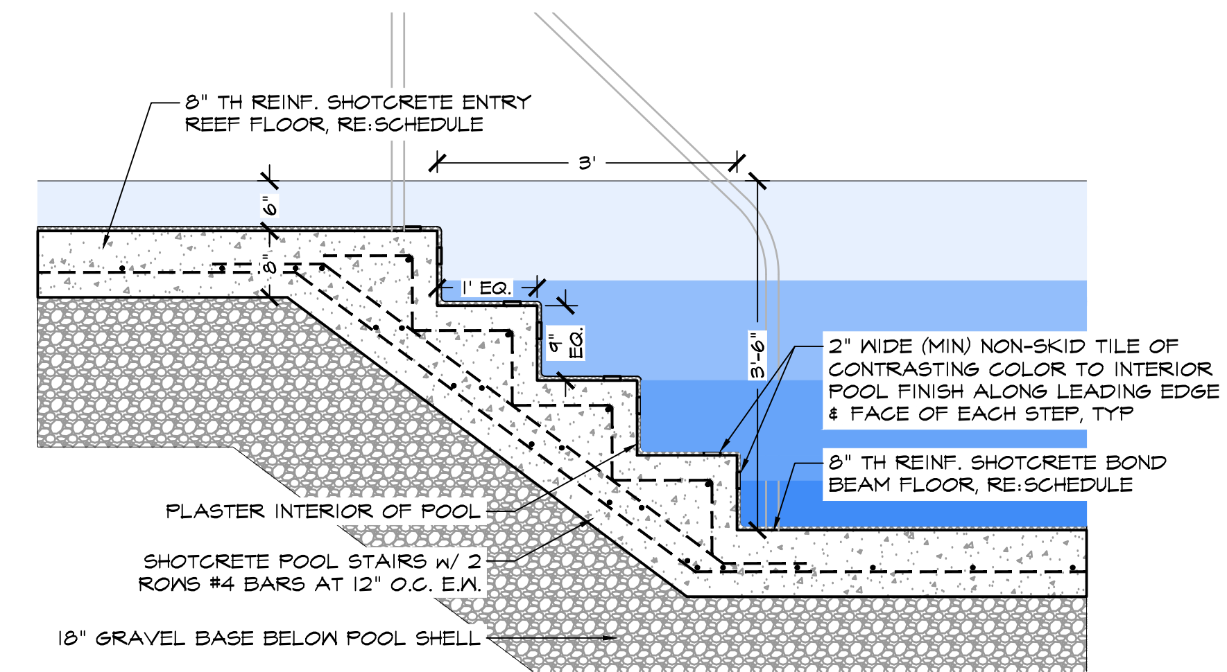
4 POOL STAIRS SCALE: 3/4" = 1'-0" SECTION
