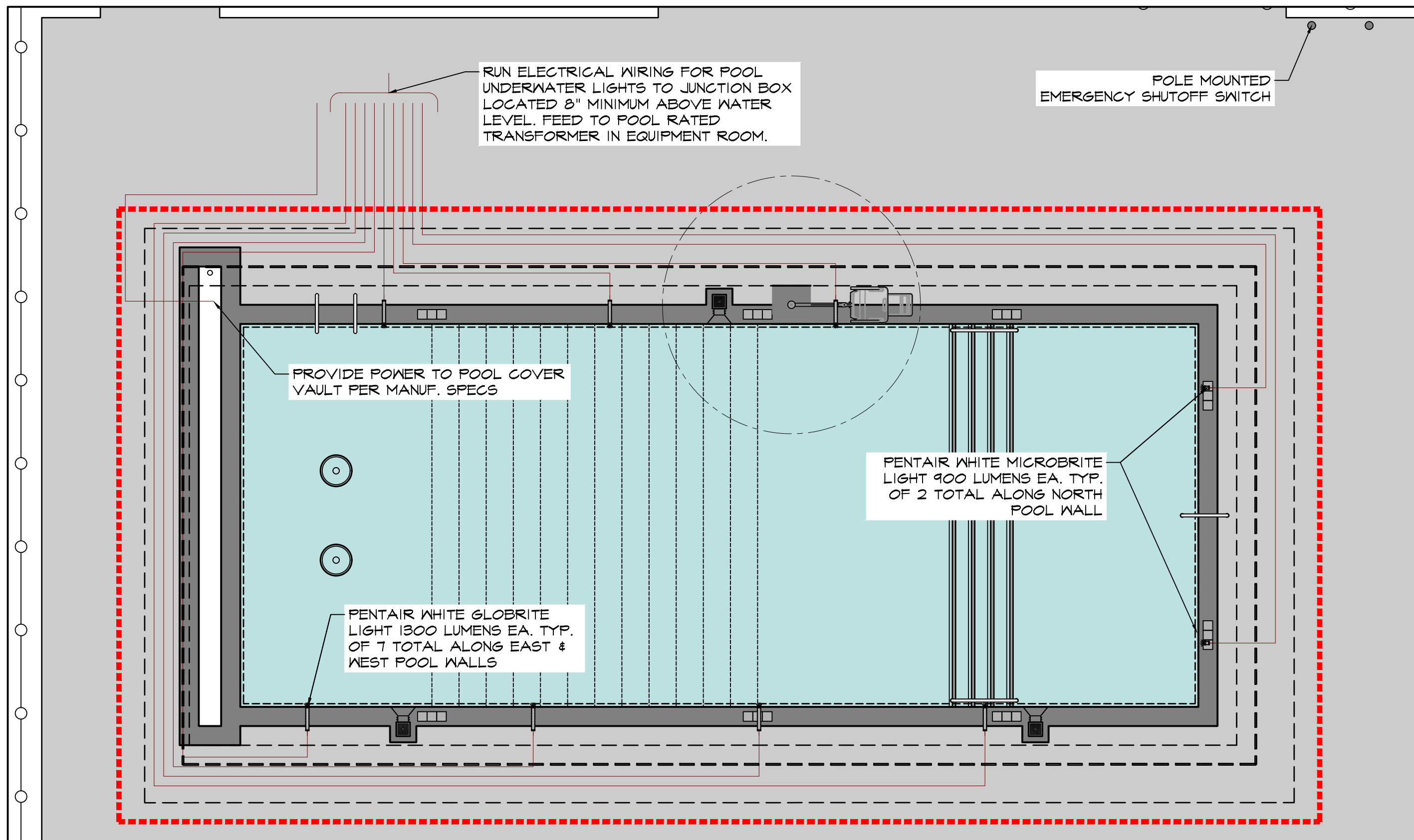
POOL ELECTRICAL PLAN SCALE: 1" = 5'-0"
