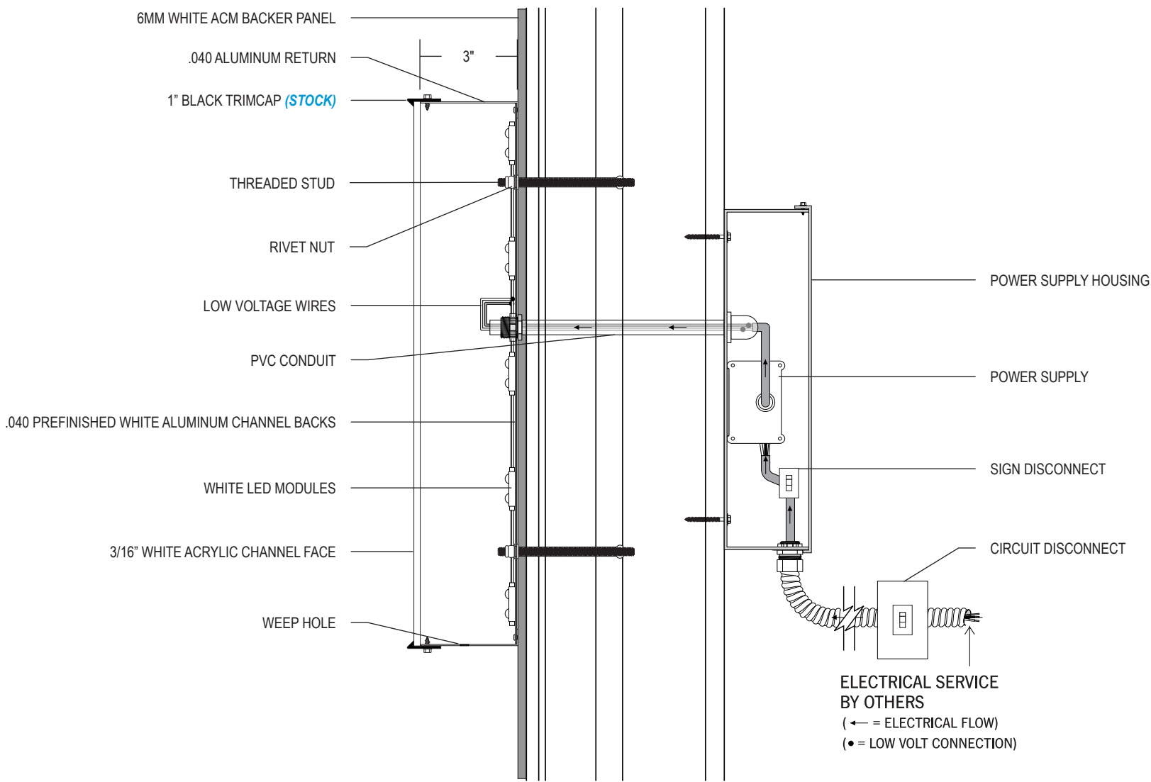
1 Channel | Flush Mount | AMC Backer | Detail Diagram ACTUAL INSTALL/WIRING MAY VARY DEPENDING UPON LOCATION CONDITIONS
