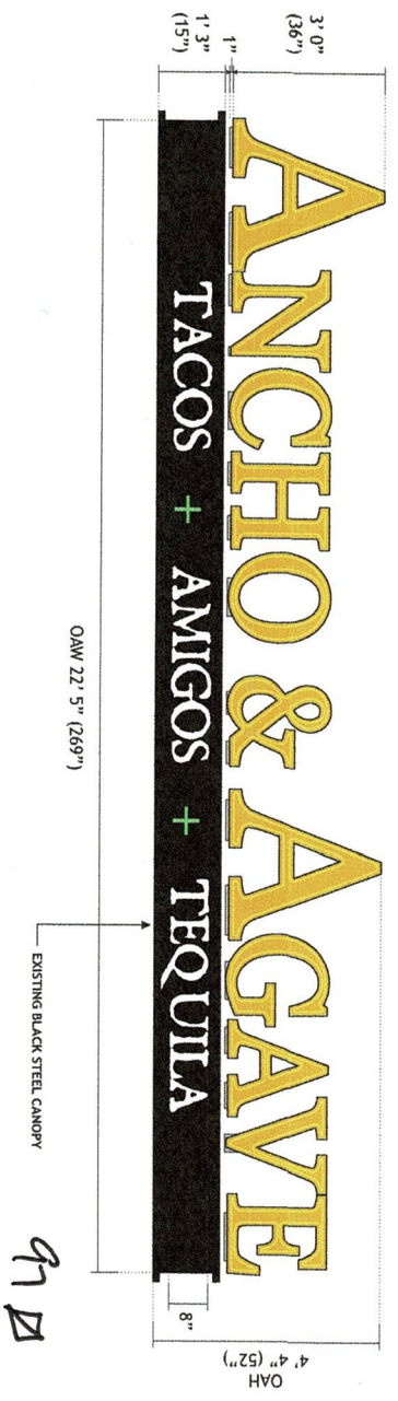
1 SIGN 1 - LAYOUT VIEW: 97.1 sf OPEN FACE FAUX NEON (LED) LETTERS W/ TAG-LINE PIN LETTERS ON CANOPY
